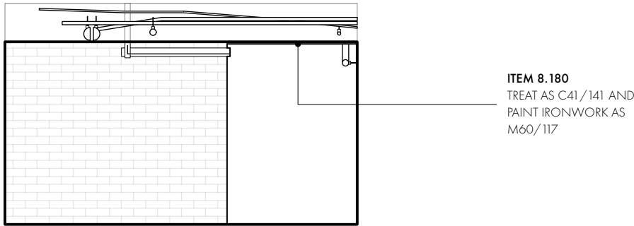
ELEVATION C
