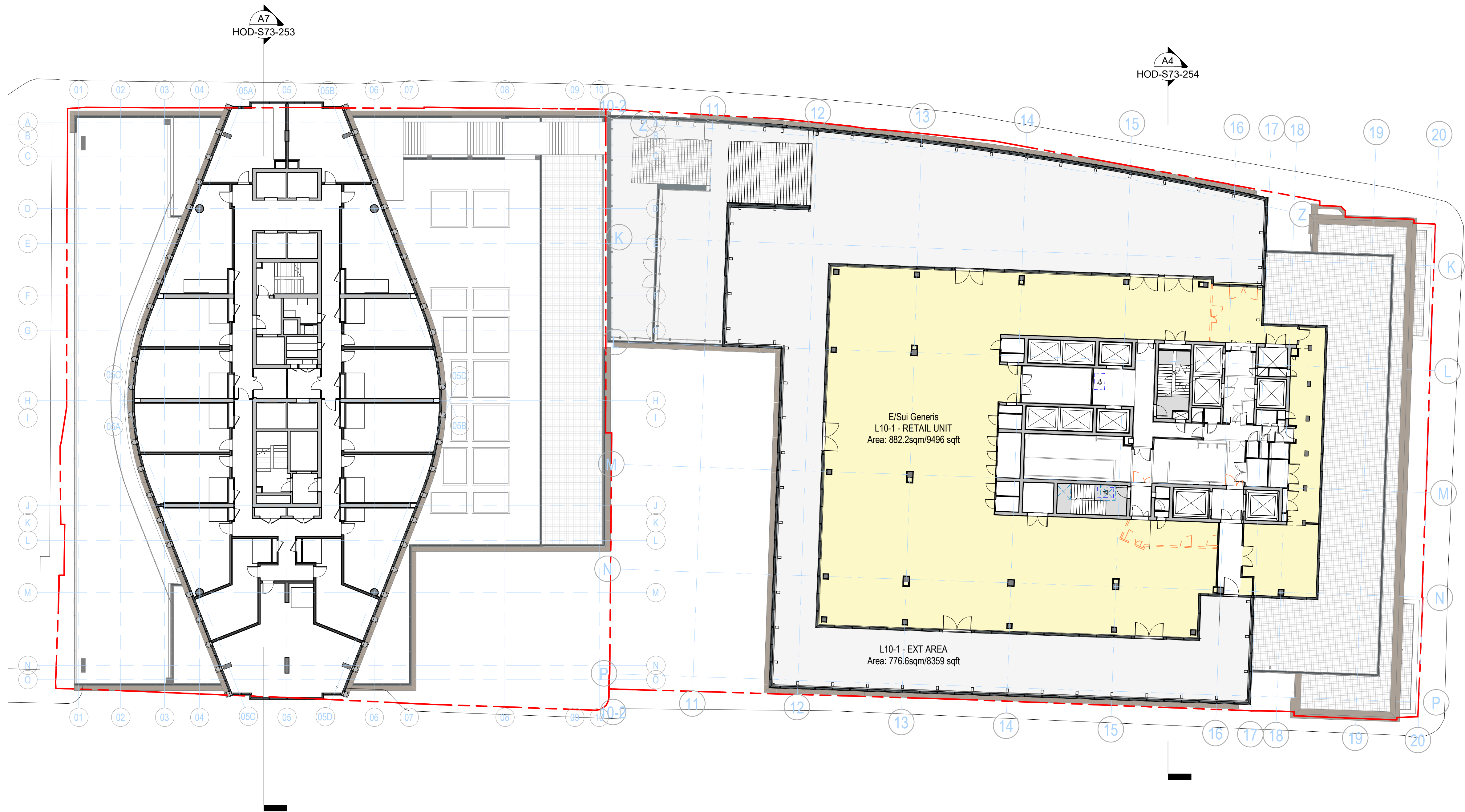
1 RETAIL PLAN - LEVEL 10 1 : 200
