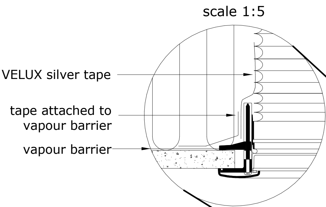
SETTING OUT
