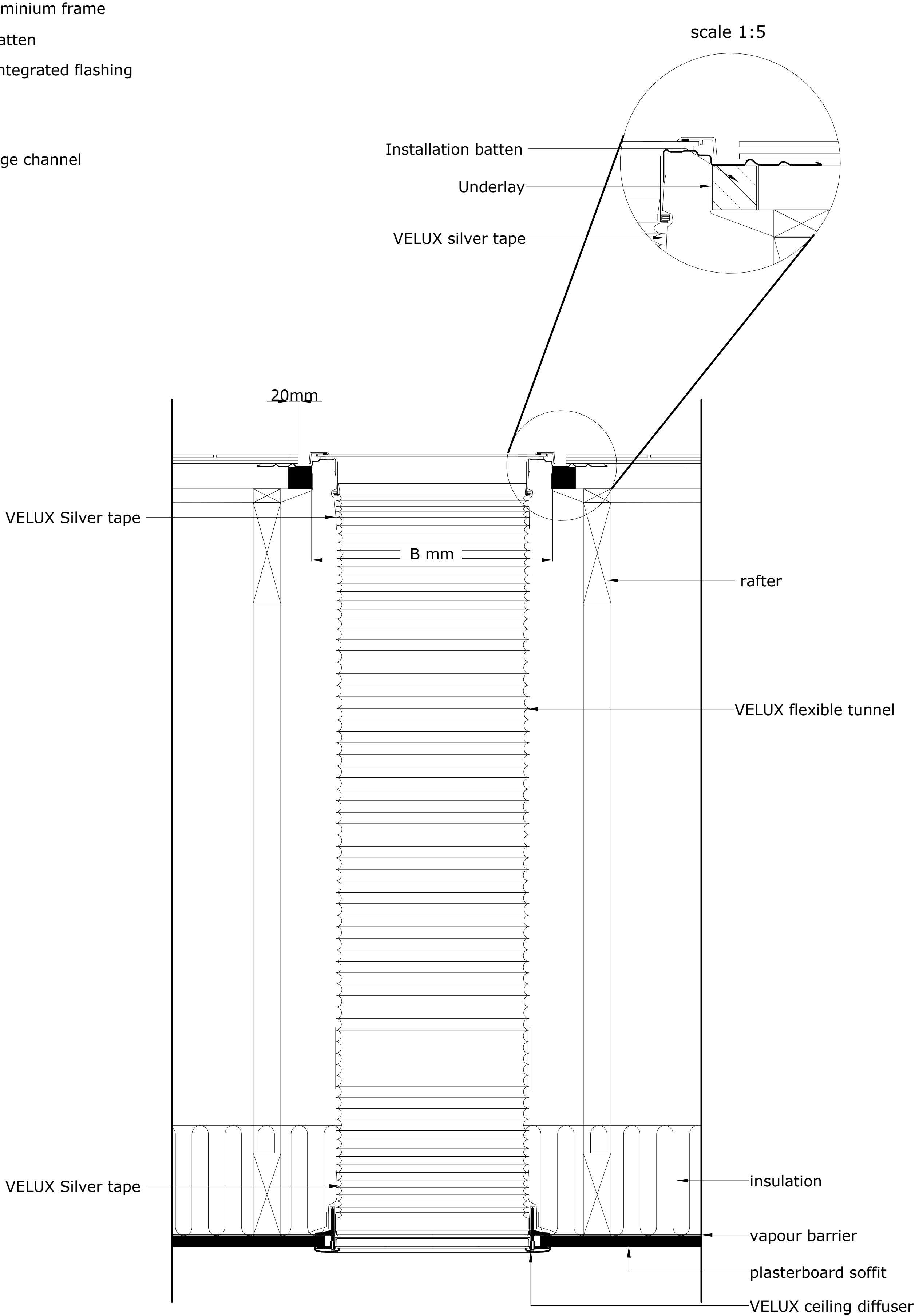
SECTION B-B
