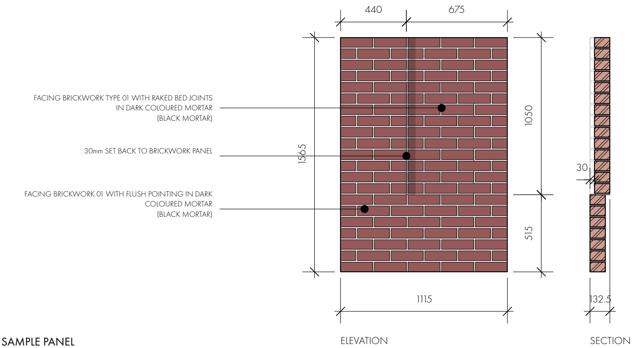
SAMPLE PANEL DEMONSTRATING KEY JUNCTIONS 1:25
