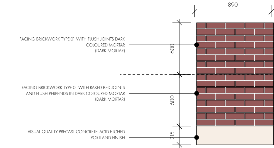
INITIAL SAMPLE PANEL TO BE CONSTRUCTED TO ESTABLISH MORTAR COLOUR AND POINTING 1:25
