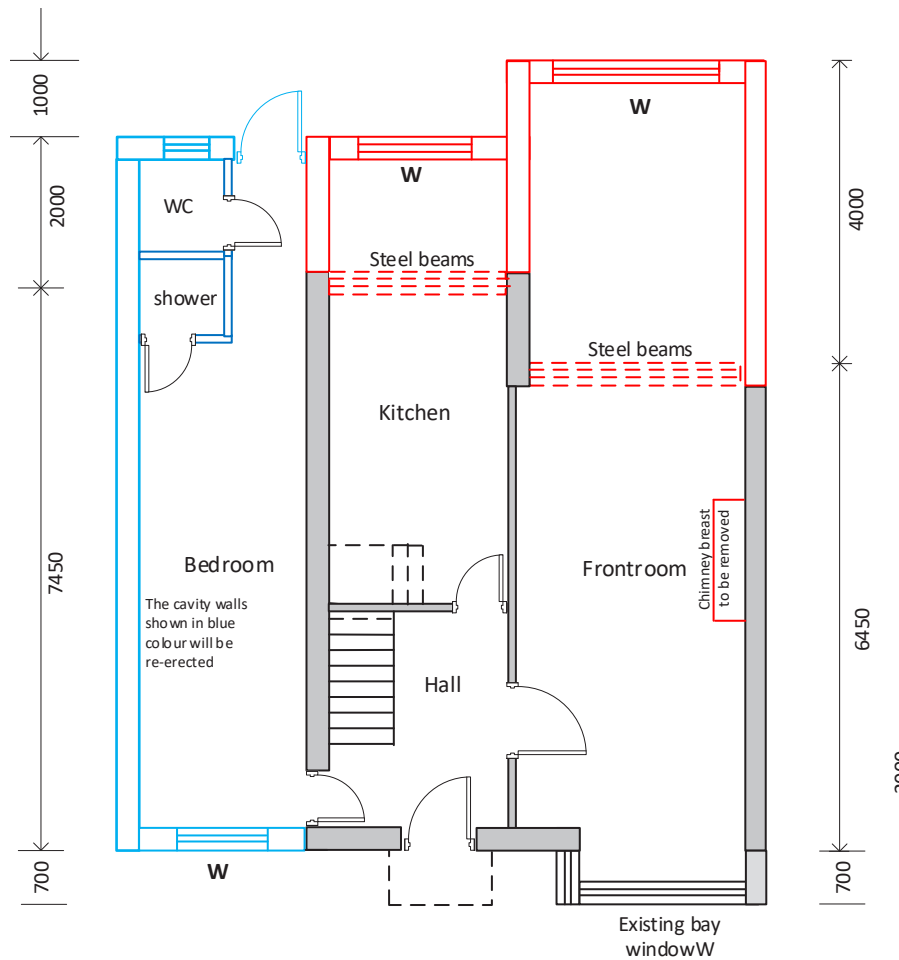
PLANNING APPROVED GROUND FLOOR PLAN 1:100 @ A3
