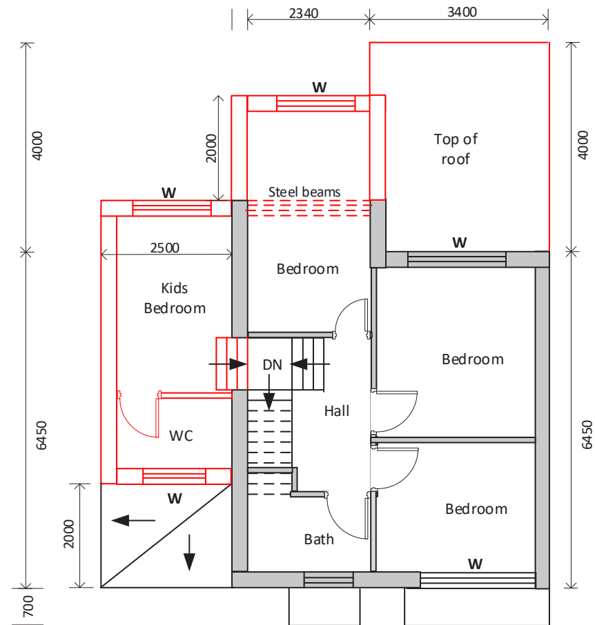
PLANNING APPROVED FIRST FLOOR PLAN 1:100 @ A3
