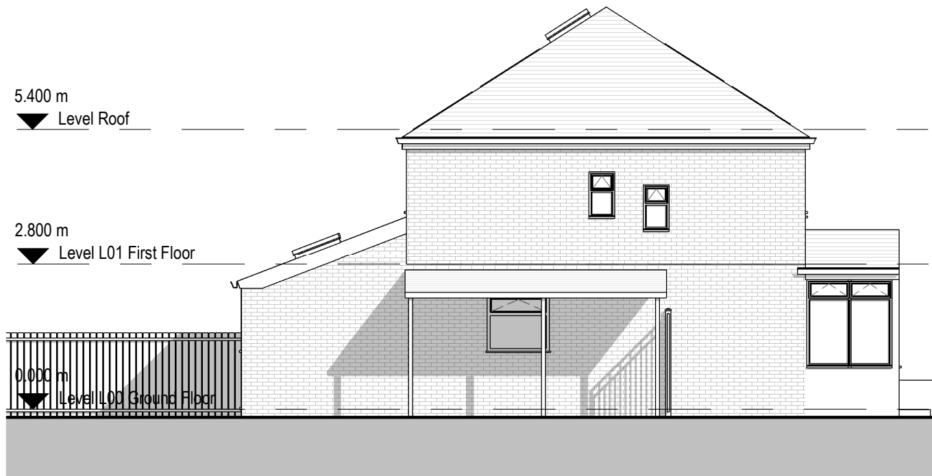
1 Existing North Elevation 1 : 100
