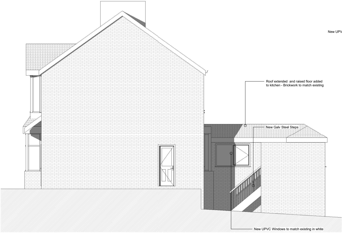
2 Proposed East Elevation
