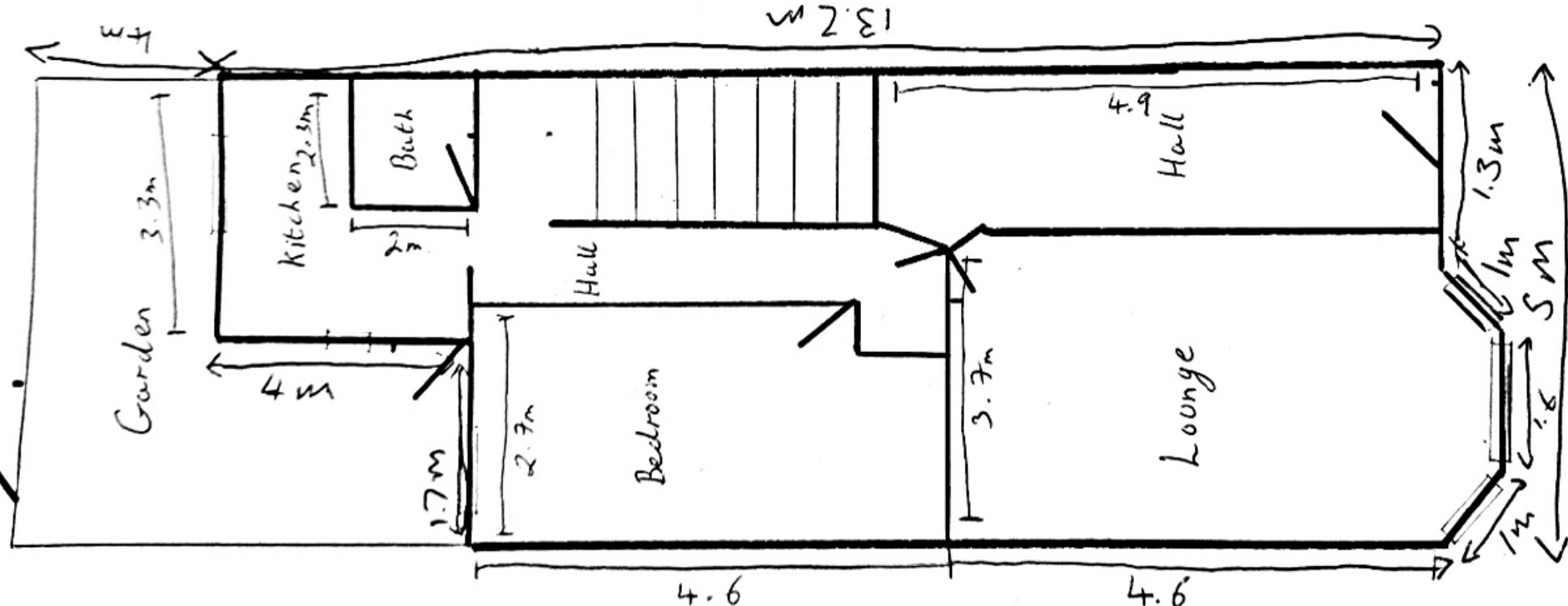
Ground Floor
