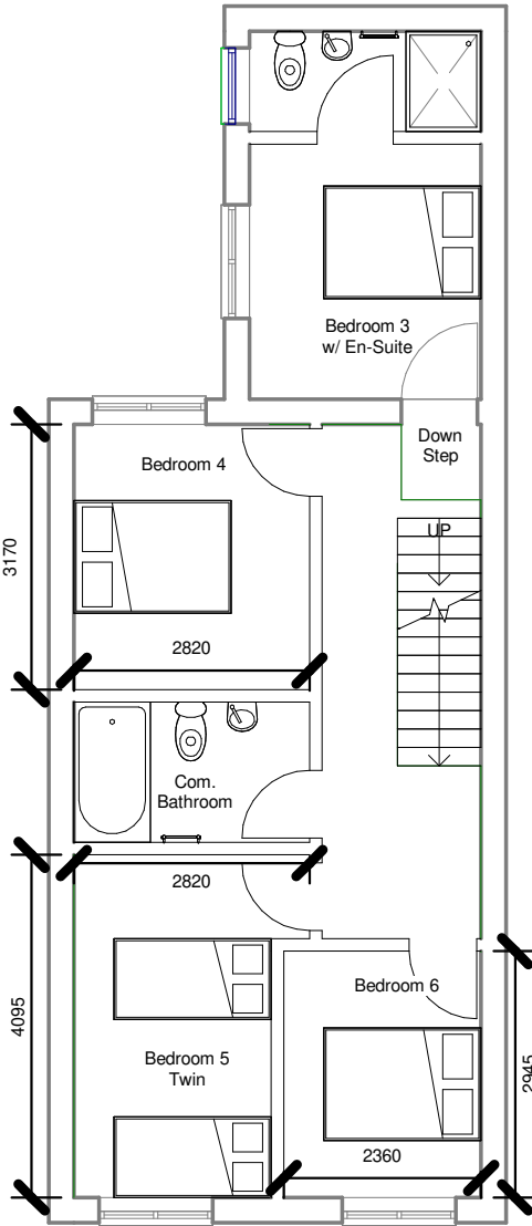
7 10 - Second Floor Plan 1 : 100
