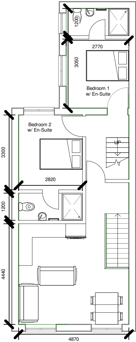
6 09 - First Floor Plan 1 : 100
