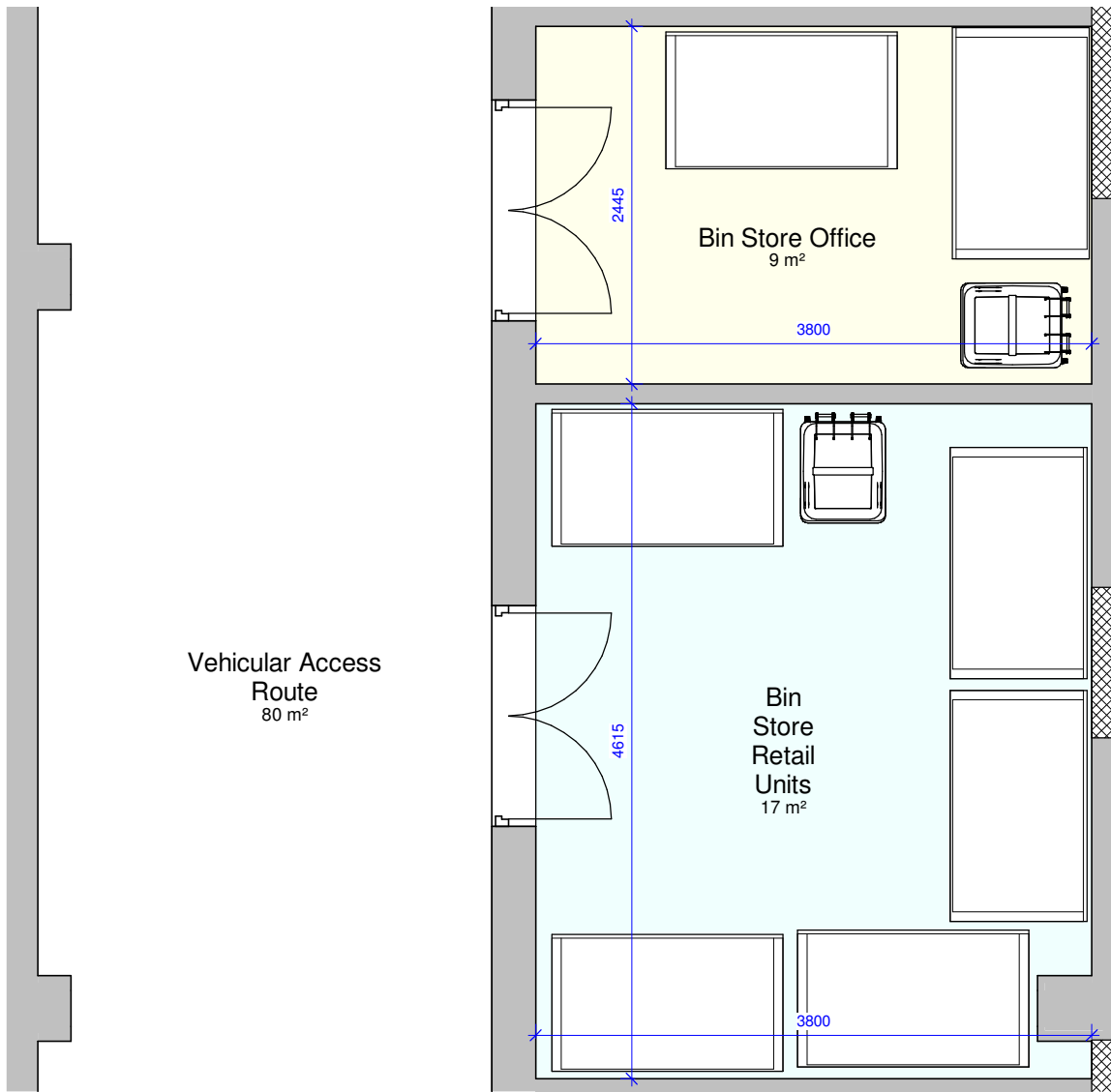
1 Proposed Bin Store Plan 1 : 50
