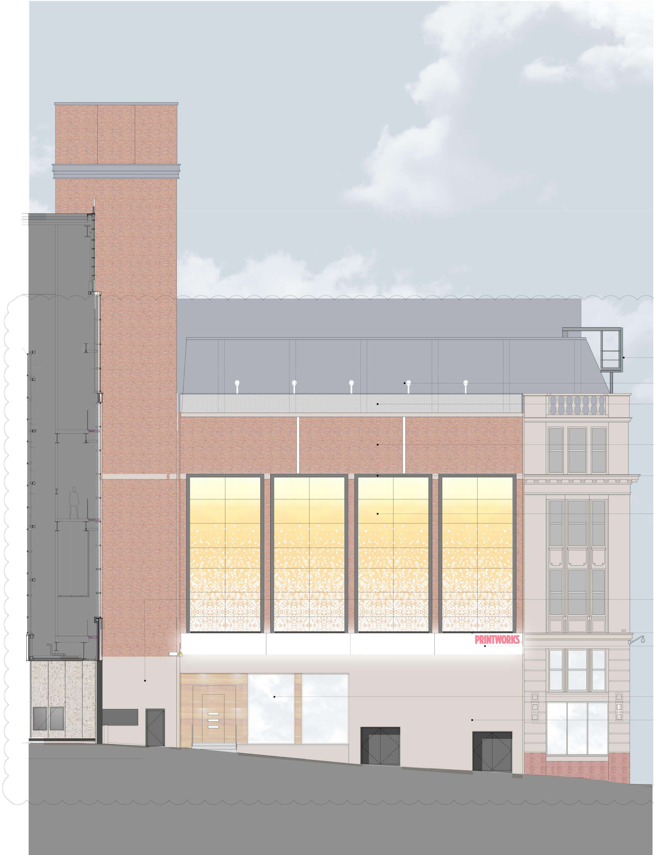
Corporation Street Return Facade and Entrance Section
