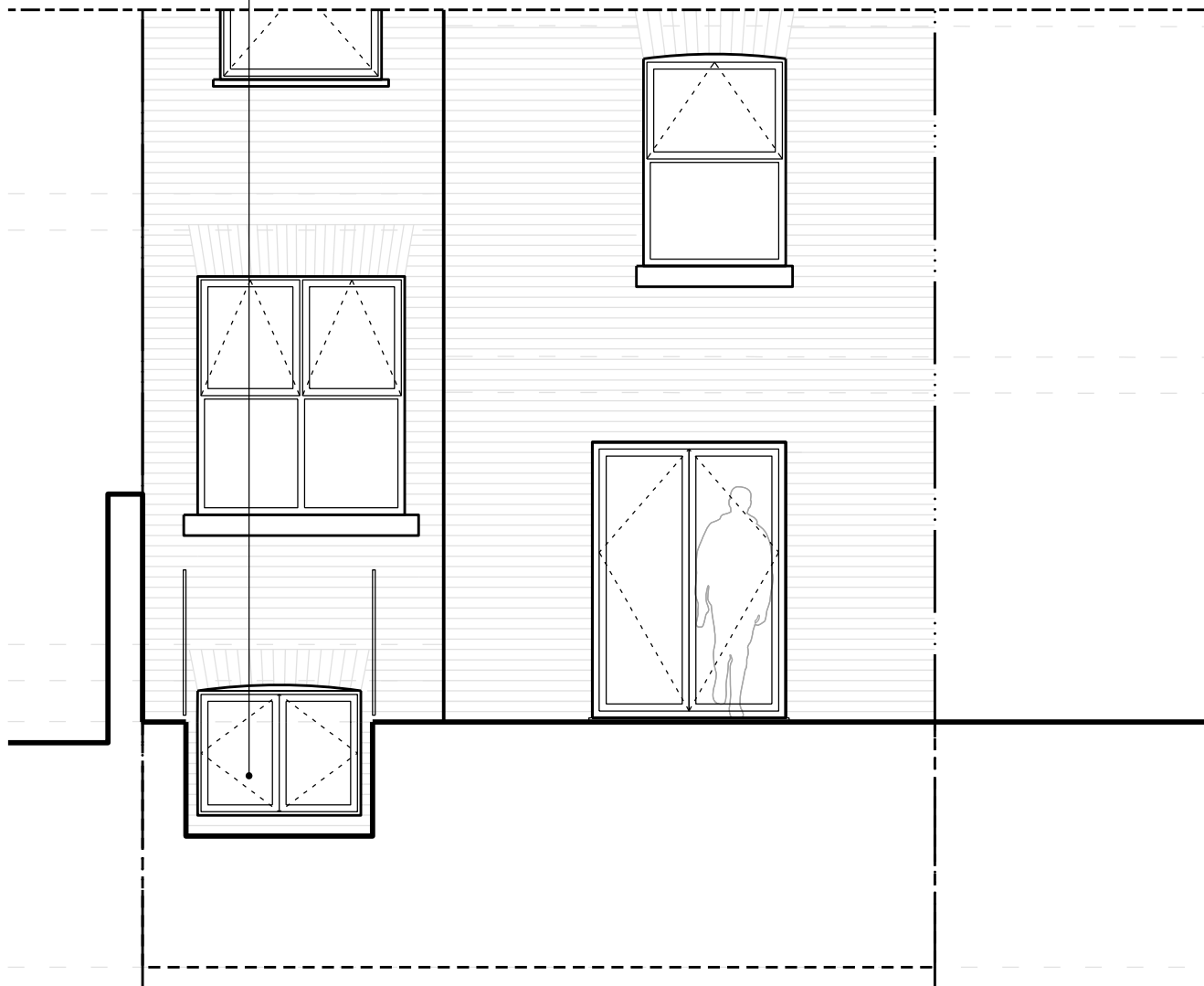
Proposed Rear Elevational Section BB
