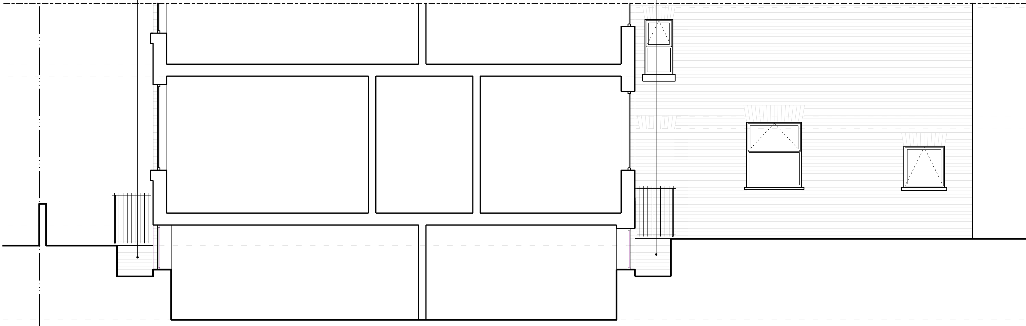
Proposed Cross Section CC
