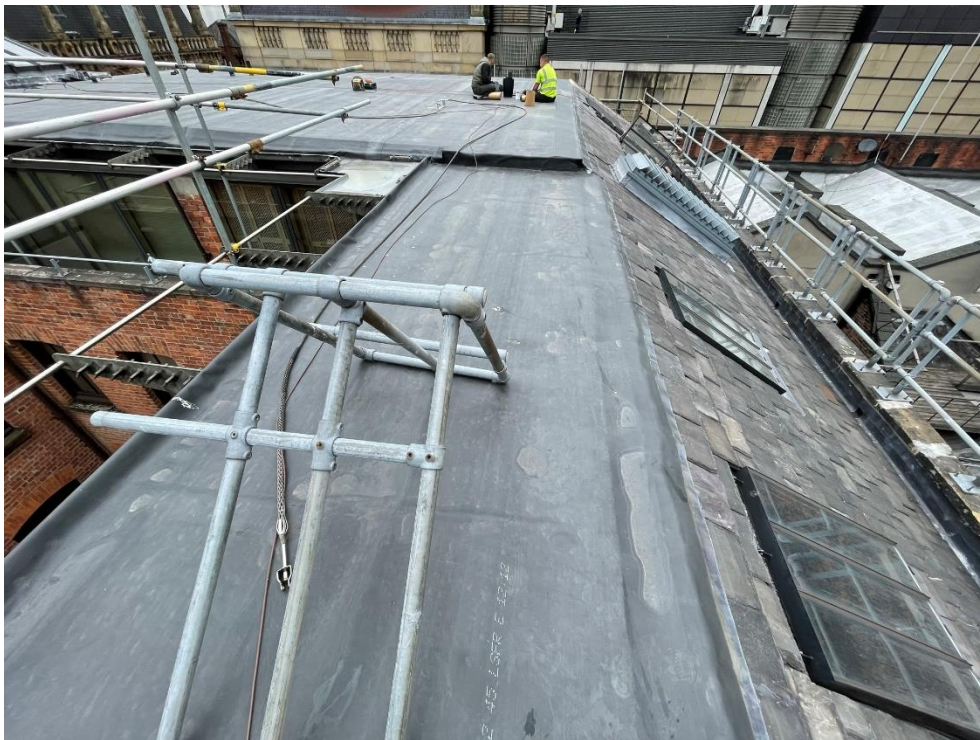
EPDM covering to main flat roof
