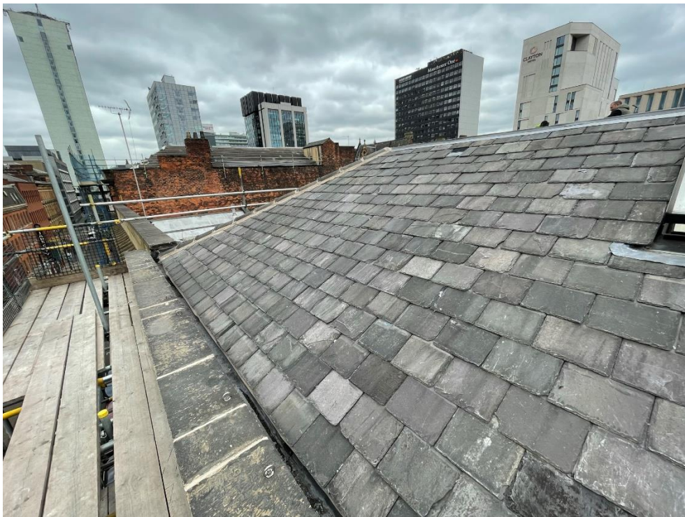
Slated mansard to George Street elevation
