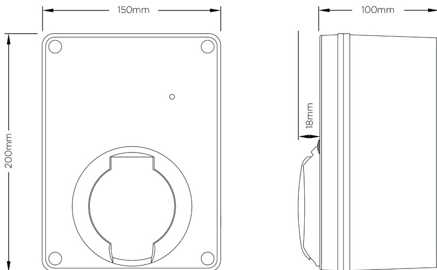
Figure 1 General Arrangement and Dimensions
