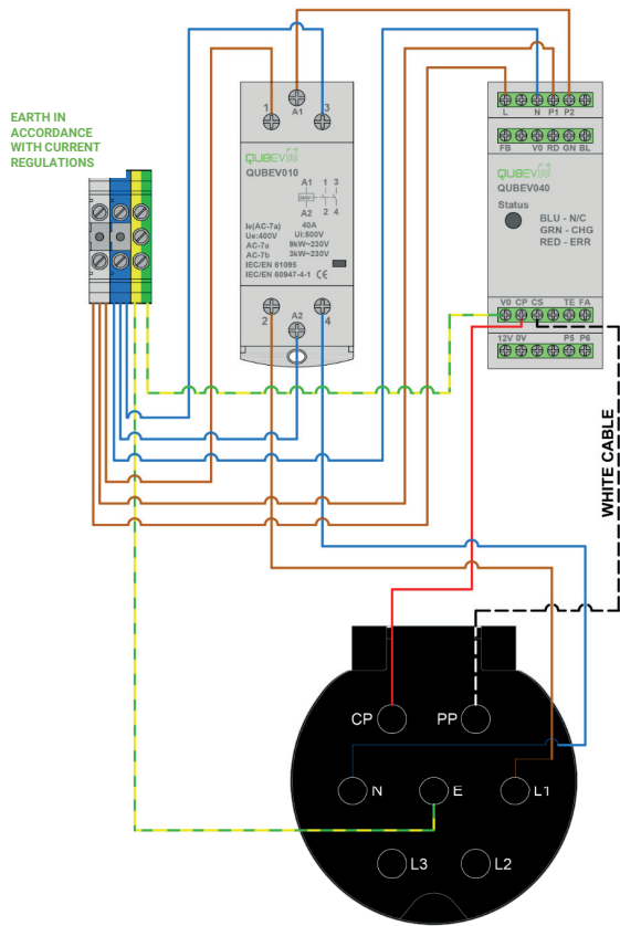
Figure 3 EVON0010 - Schematic Diagram
