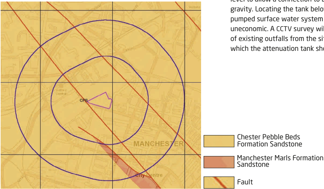
Figure 3.4 Bedrock Geology
