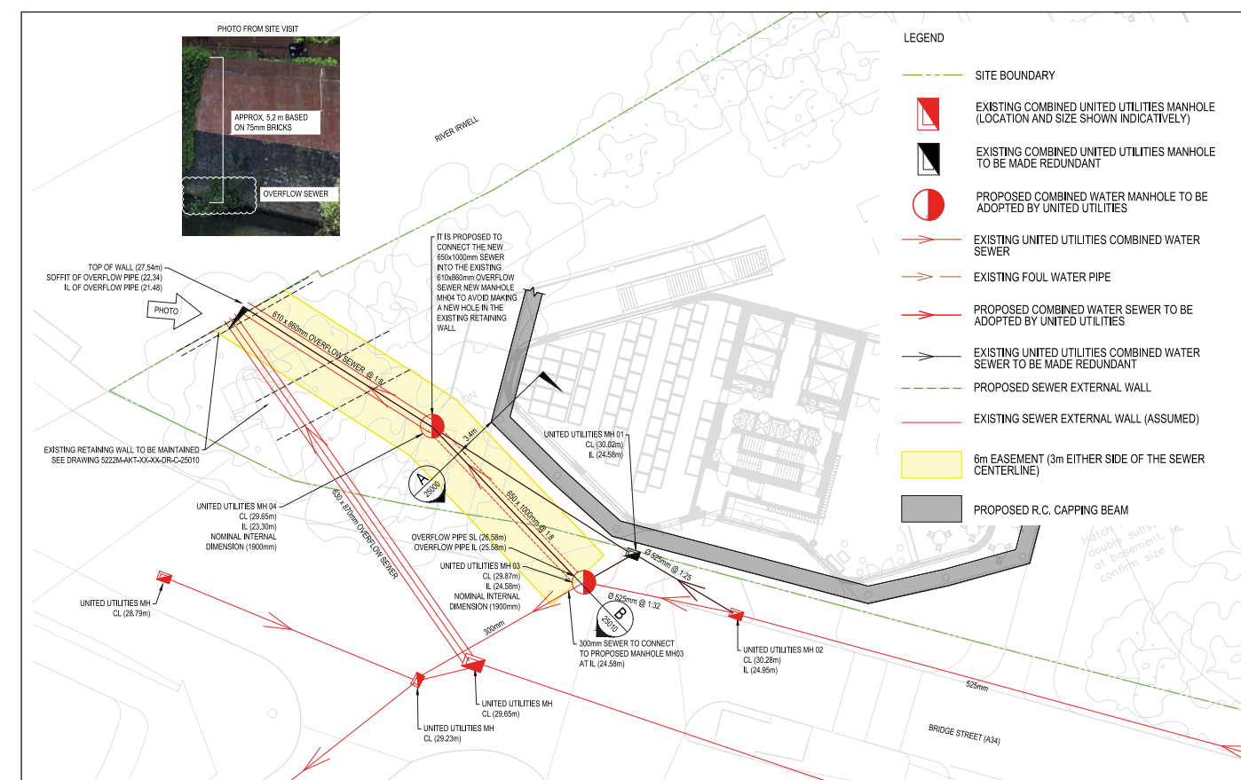
Figure 6.3 Proposed combined water overflow diversion
