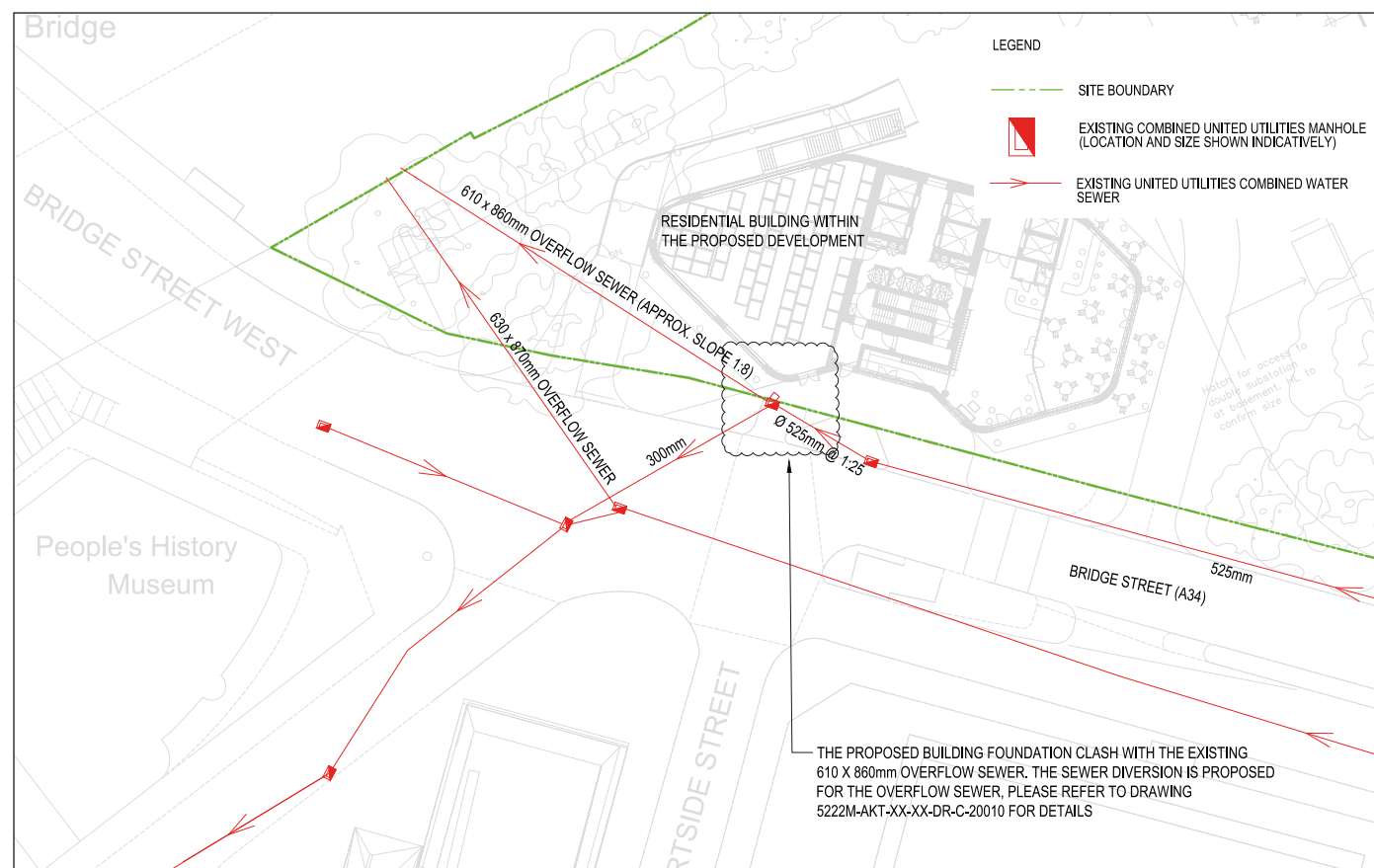
Figure 6.2 Clashes between basement and United Utilities Asset Map
