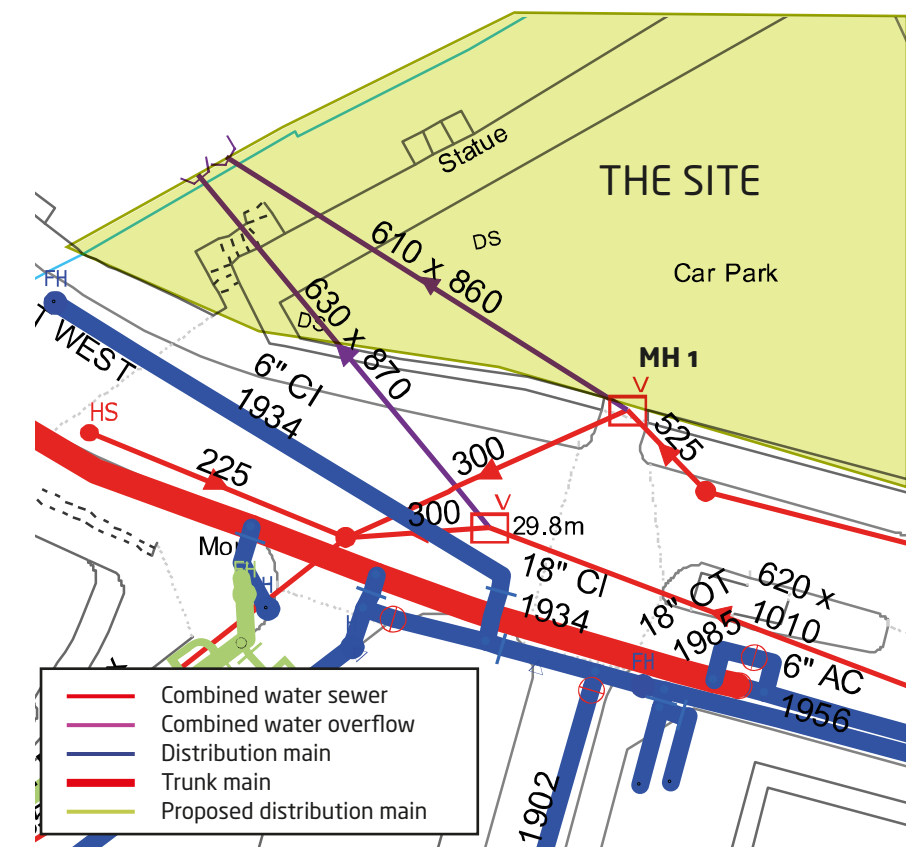
Figure 6.1 United Utilities Asset Map / combined overflow pipes
