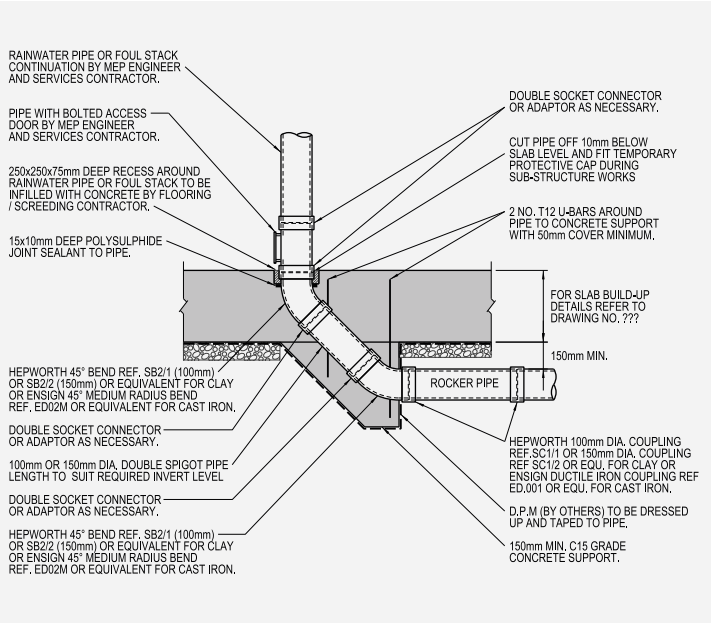
Figure 8.1 Rodding /jetting access detail
