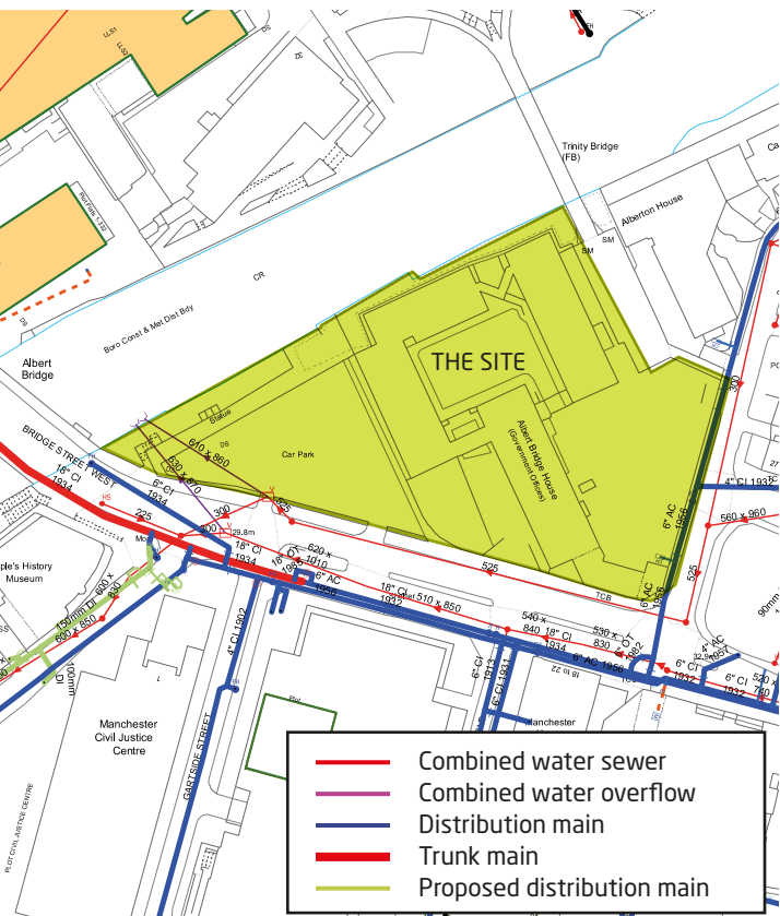
Figure 3.1 United Utilities Sewer Record
