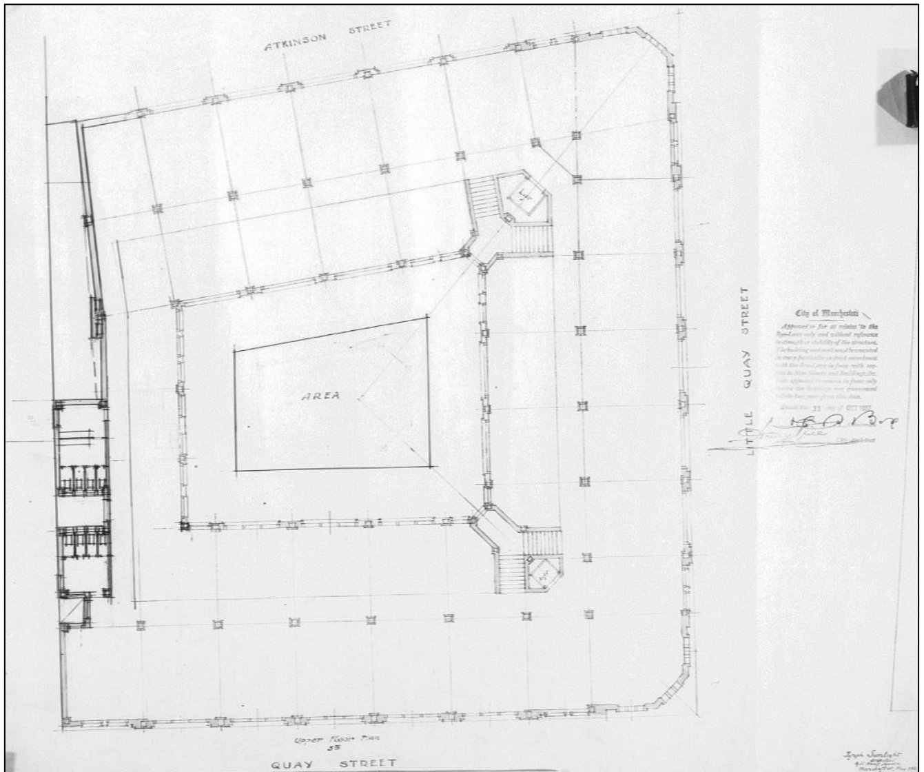
Image G: Fifth floor plan (1927)
