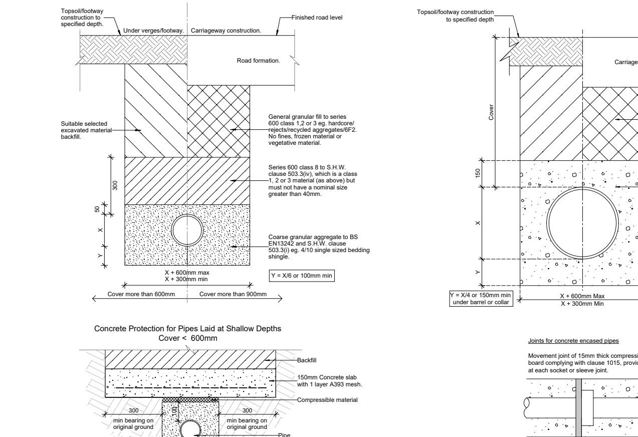
Pipe Bedding Detail Type Z
