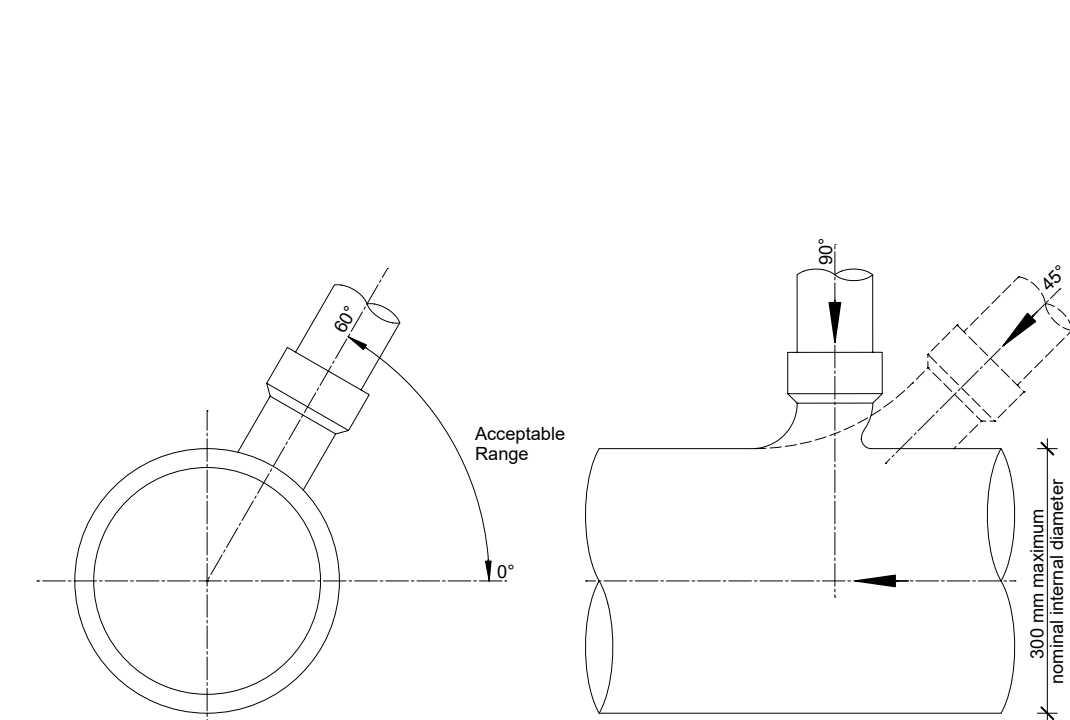
Cross-Sectional View of Sewer
