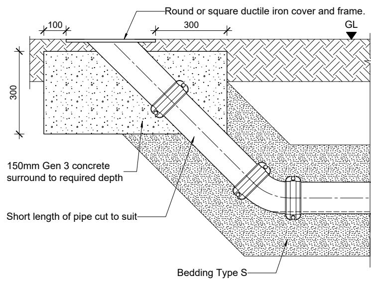
External Rodding Eye Detail
