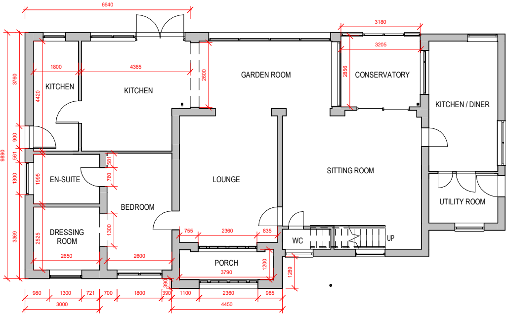
1 Ground Floor 1 : 150
