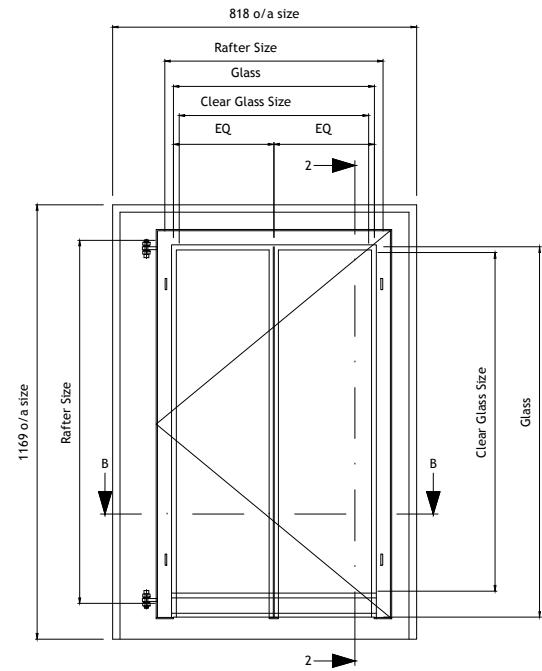
TILE ROOF APPLICATION
