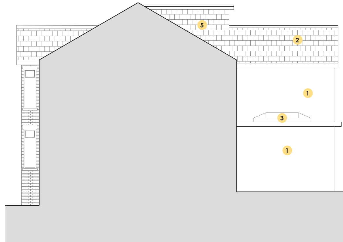
PROPOSED SIDE ELEVATION 1:100 @ A3
