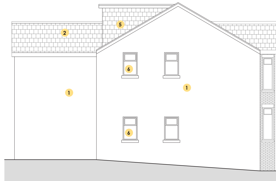
APPROVED SIDE ELEVATION 1:100 @ A3
