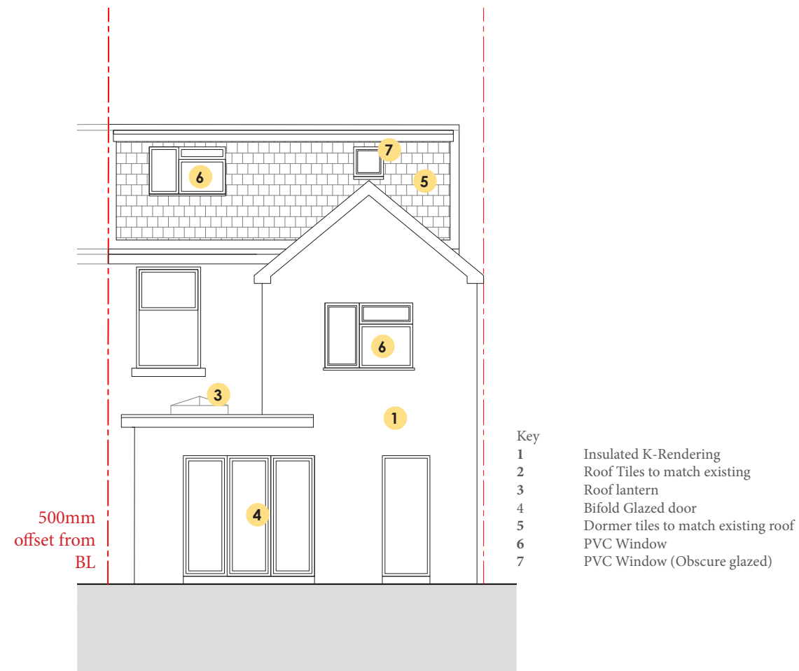
PROPOSED PROPOSED REAR ELEVATION 1:100 @ A3
