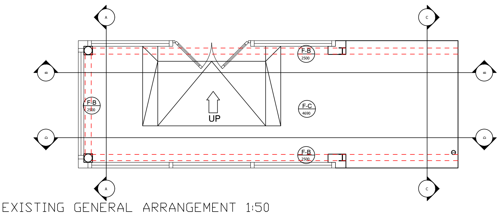
EXISTING GENERAL ARRANGEMENT 1:50
