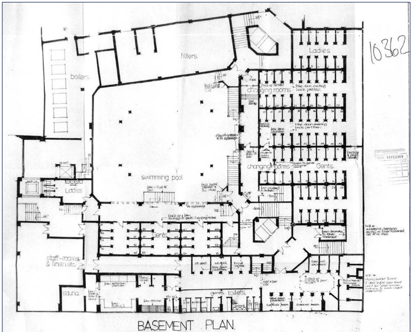
Figure 13 - Proposed basement plan submitted as part of the 1979 consented application.
