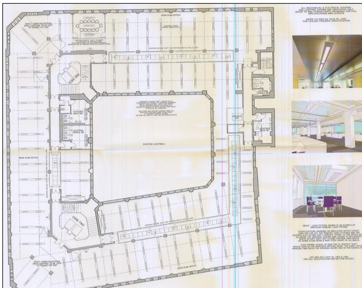
Figure 26 - Indicative proposed ceiling plan/lighting scheme submitted as part of the 2008 application (087147/LO/2008/C1).
