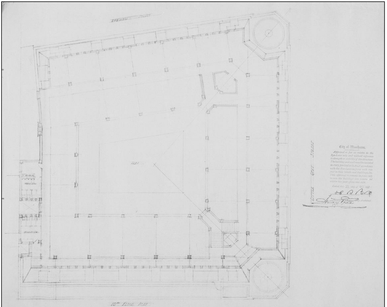
Image J: Tenth floor plan (1927)
