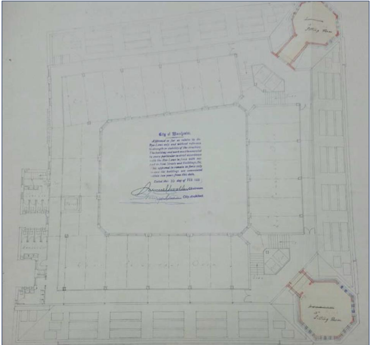
Image N – Thirteenth floor plan (1931)
