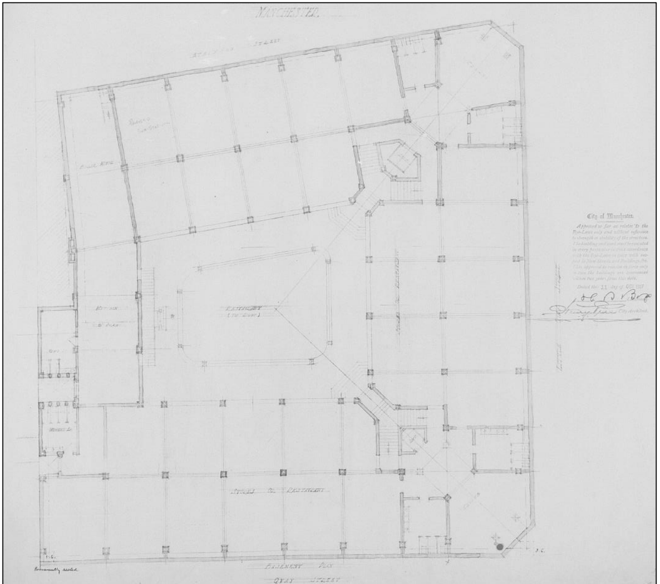
Image A: Sub-basement plan (1927)
