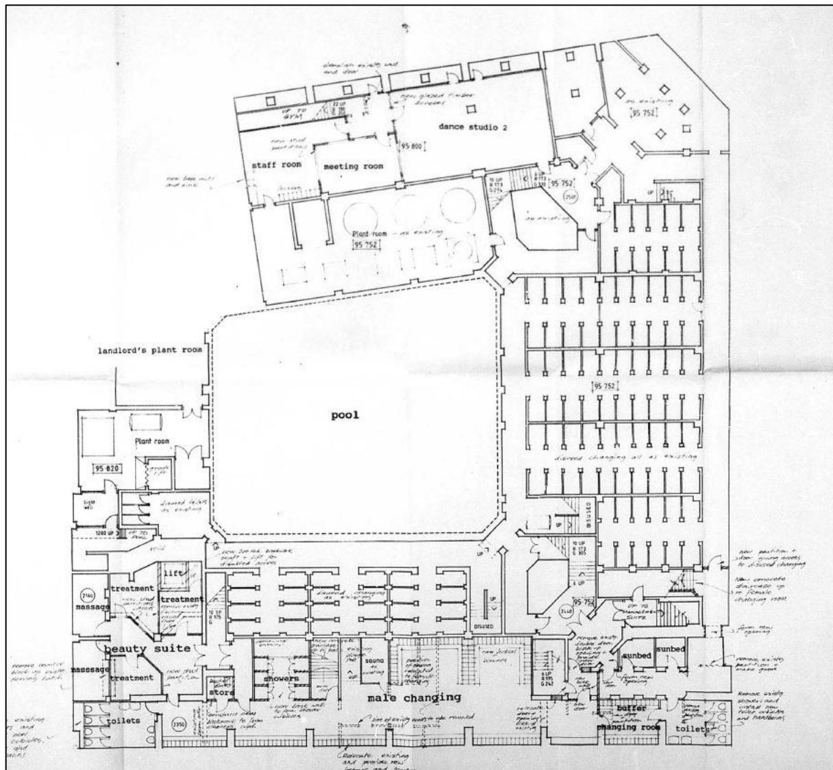
Figure 20 - Proposed sub-basement plan submitted as part of the 1995 application.
