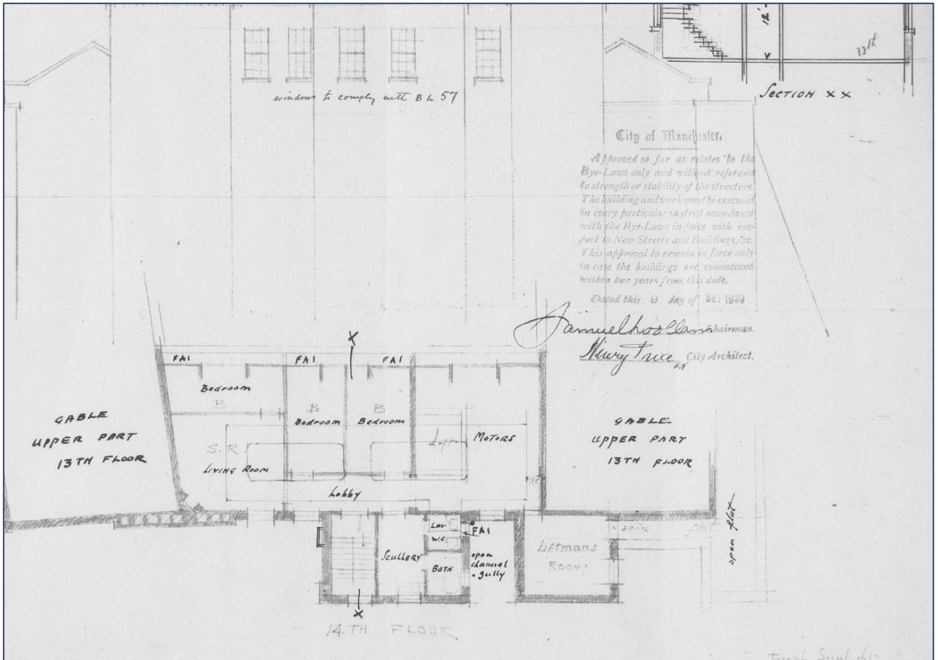
Image O – 1939 caretaker's flat floor plan (fourteenth floor)
