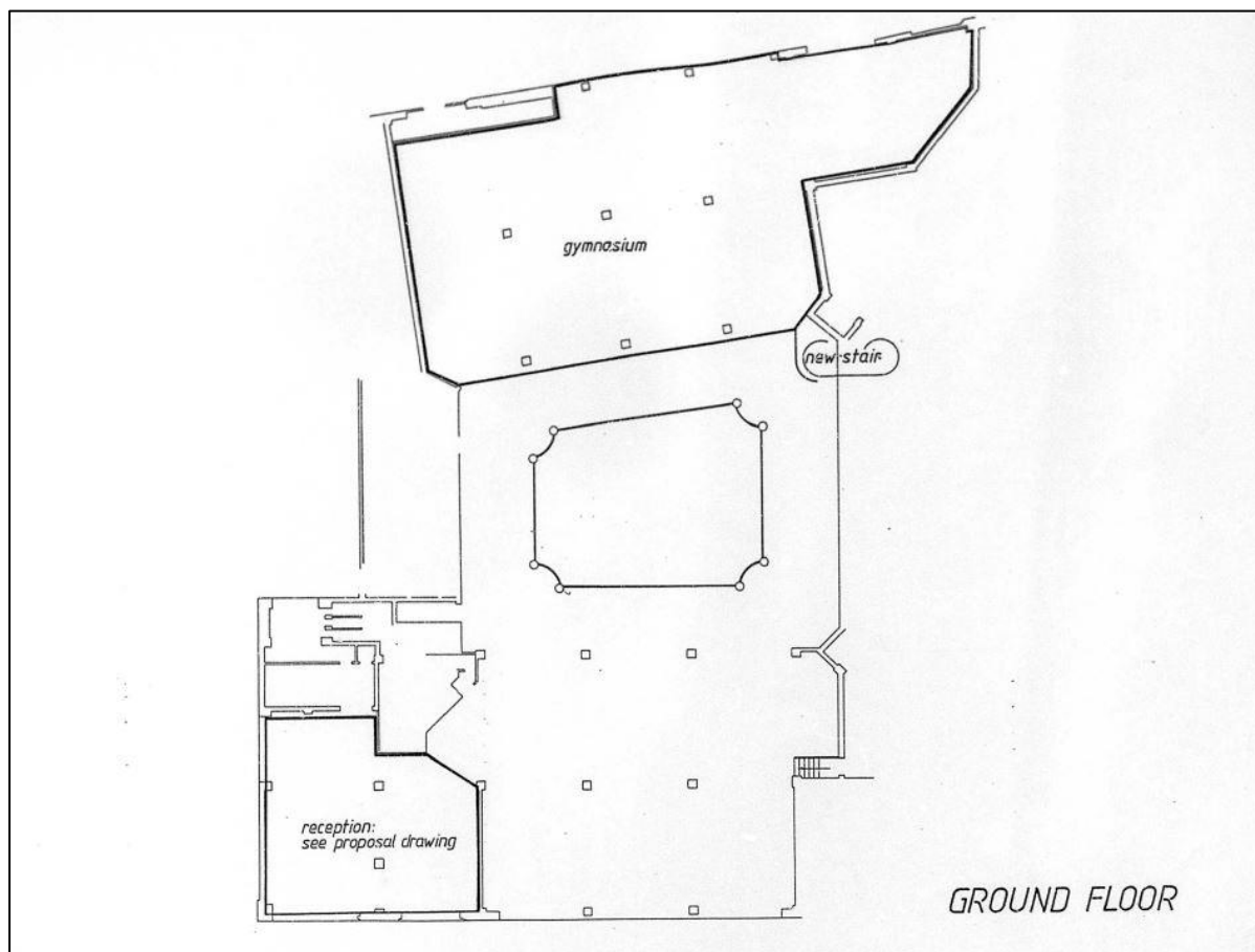
Figure 24 - Proposed ground floor plan, submitted as part of the 1995 consented application.
