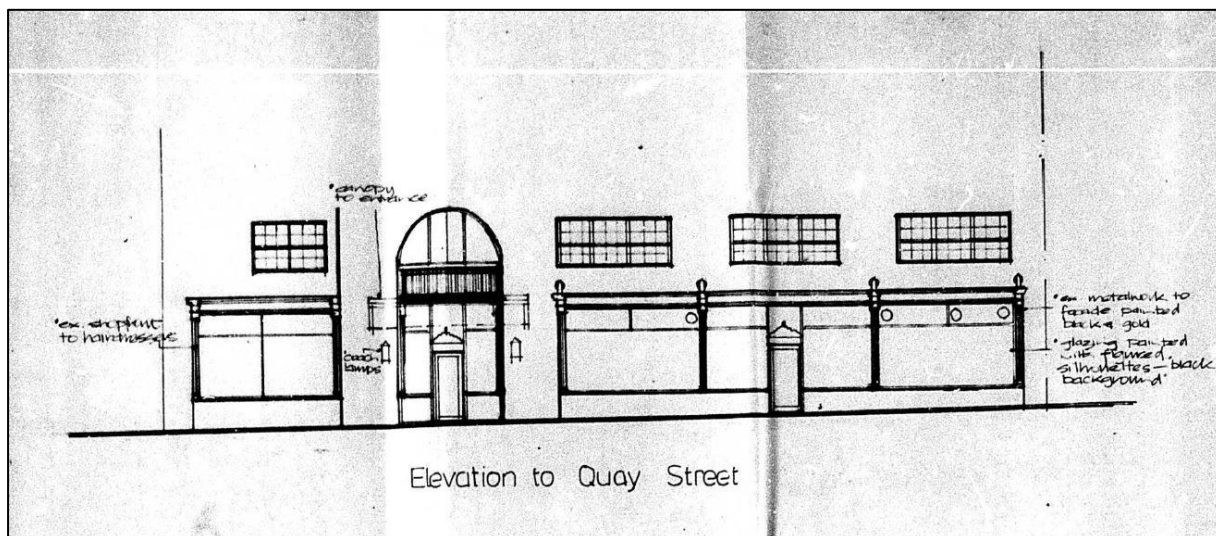
Figure 15 – Proposed changes to Quay Street elevation, submitted as part of the 1979 consented application.
