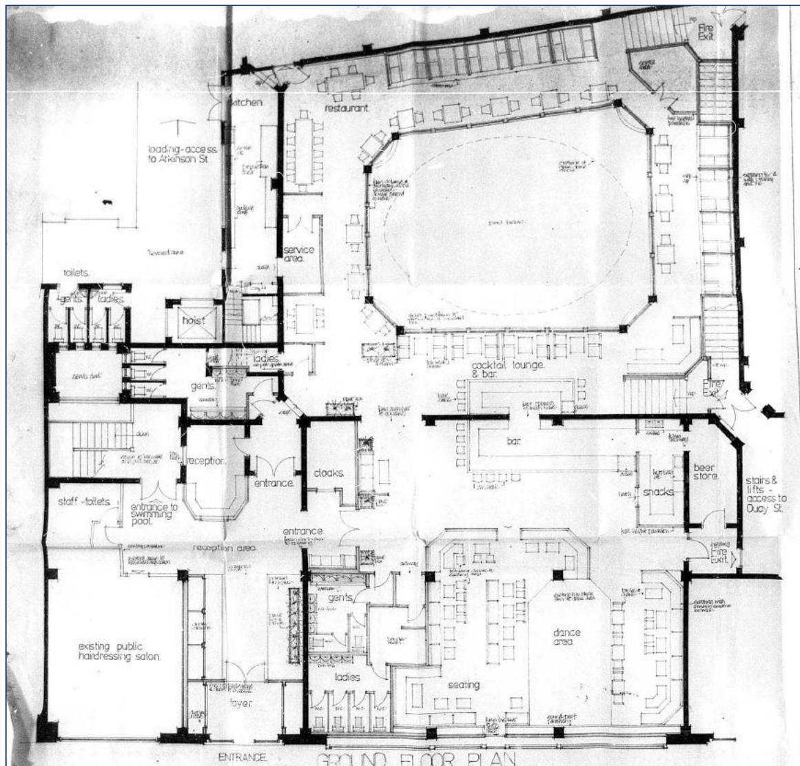
Figure 14 - Proposed ground floor plan submitted as part of the 1979 consented application.
