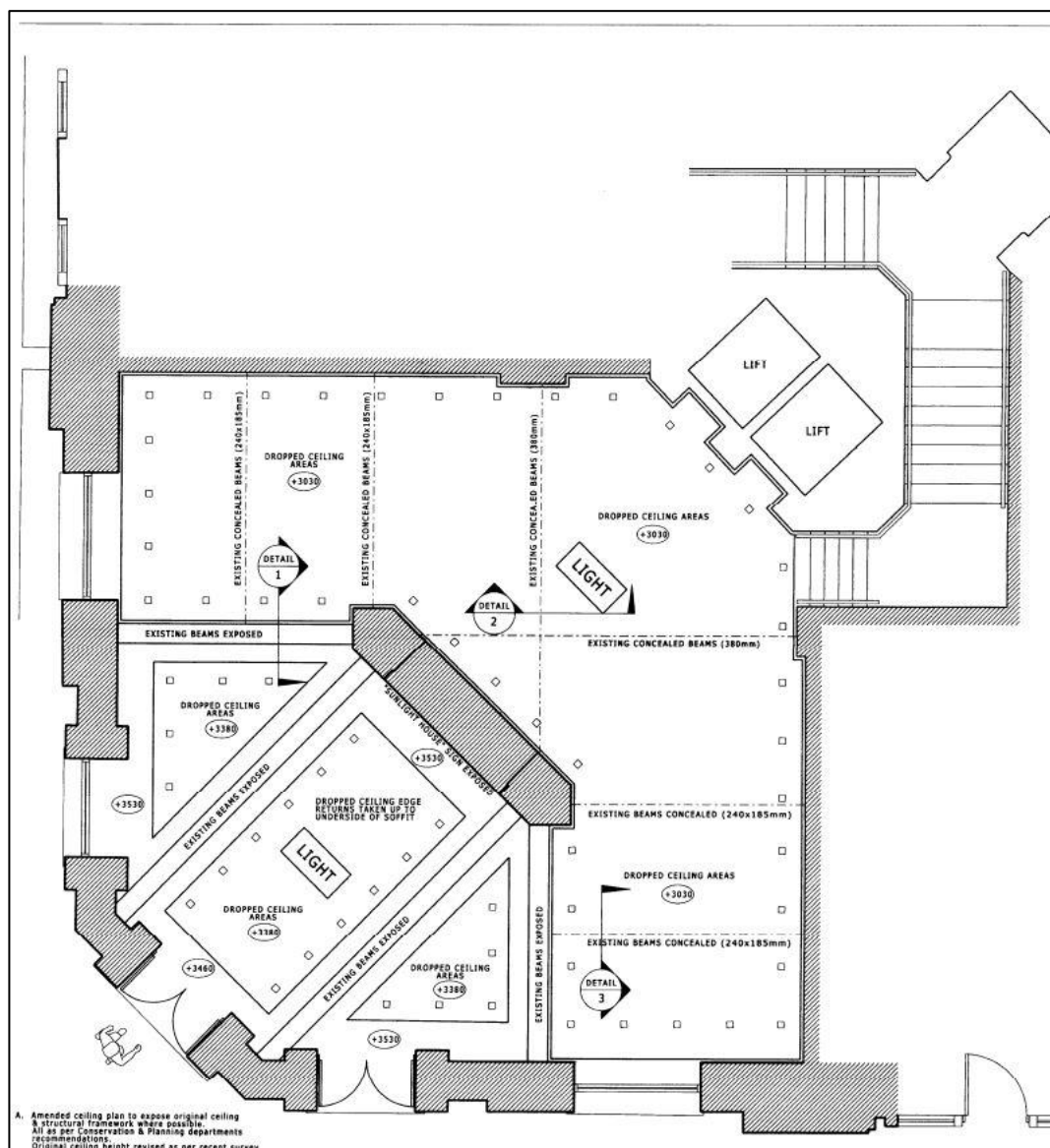
Figure 25 - Proposed changes to reception submitted as part of the 2008 application (085698/LO/2008/C1).
