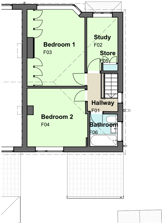
2 01-First Floor 1:100
