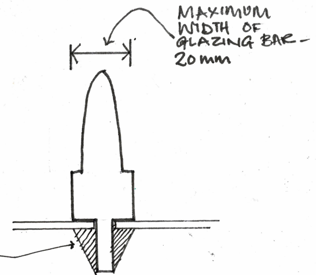
CROSS SECTION DETAIL OF LAMB'S TONGUE GLAZING BAR [common to all windows] SCALE - 1:1 @ A3
