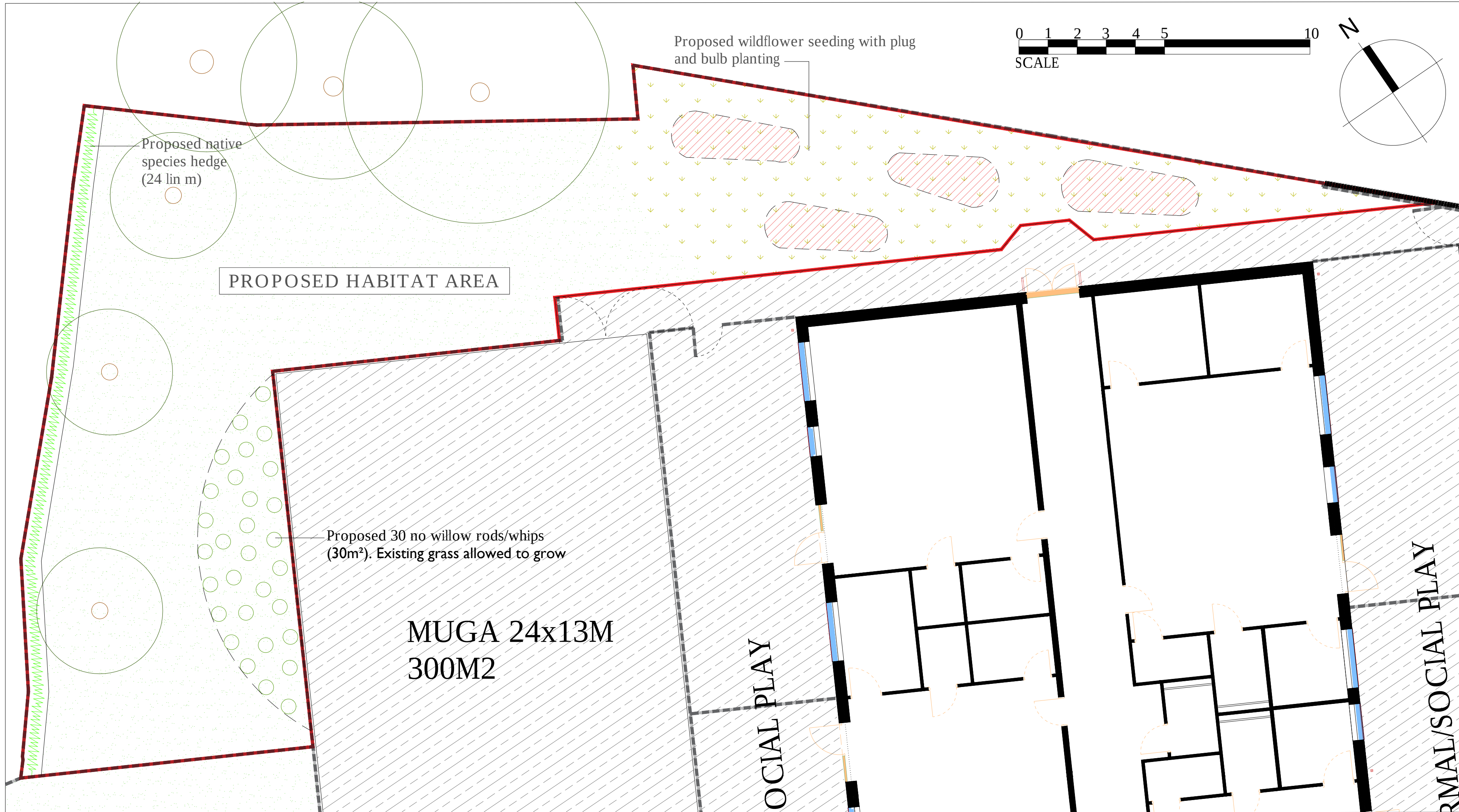
PROPOSED RELOCATED HABITAT AREA SCALE 1:100
