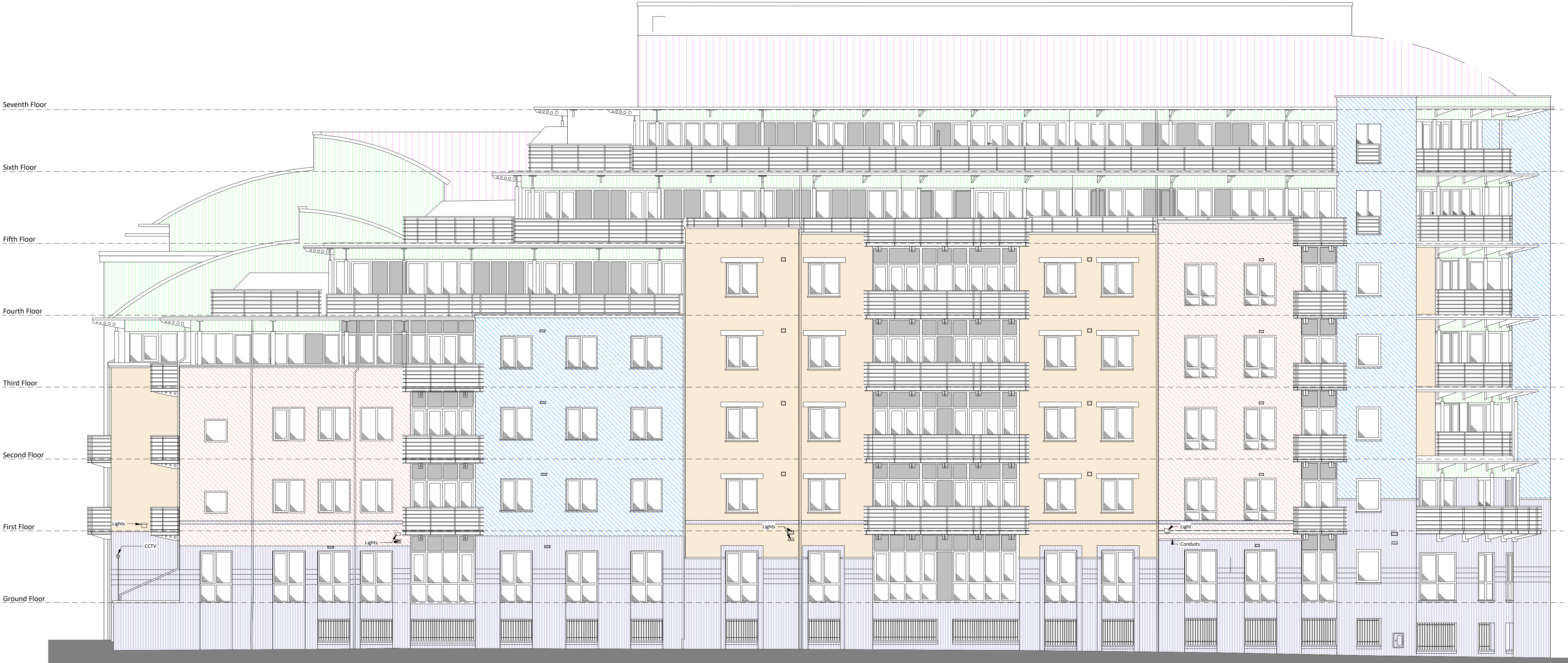
Elevation 4 (Shortcroft Street) 1 : 100
