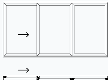
Three pane Single track slide XOO / OOX
