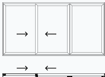
Three pane Double track lift and slide XXO (Type1) / OXX (Type1)
