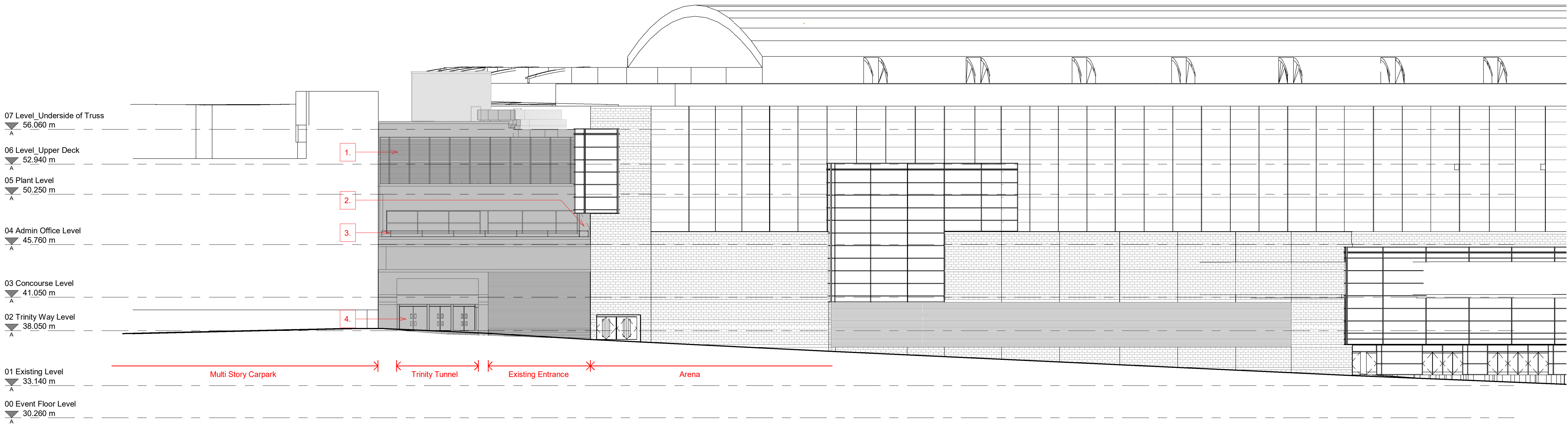
2 Planning Elevation - Proposed Trinity Way Elevation 1 : 200
