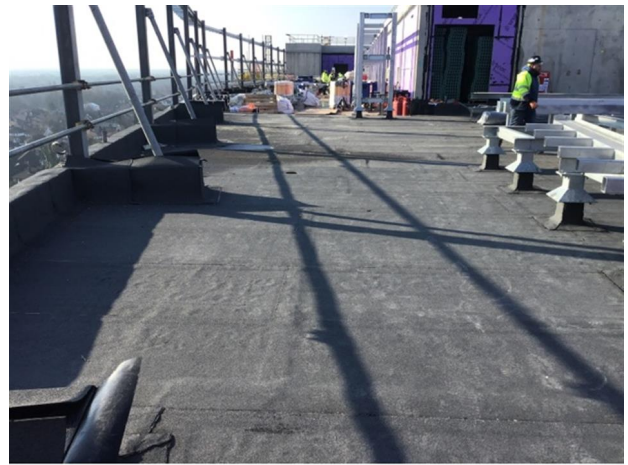
Photo 4 - View of cap sheet to section 3
