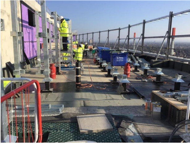
Photo 1 - Overview of level 9 section 2
