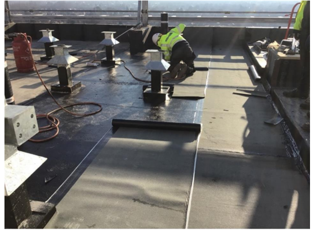
Photo 2 - View of AVCL being installed
