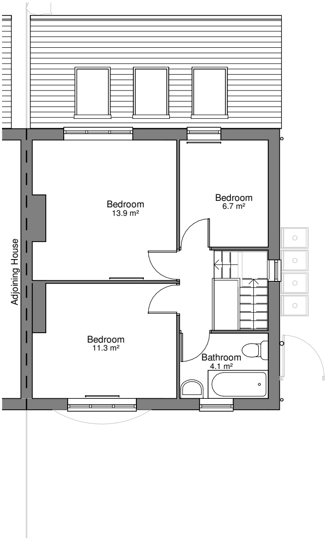
First Floor Plan - Proposed 1 : 100
