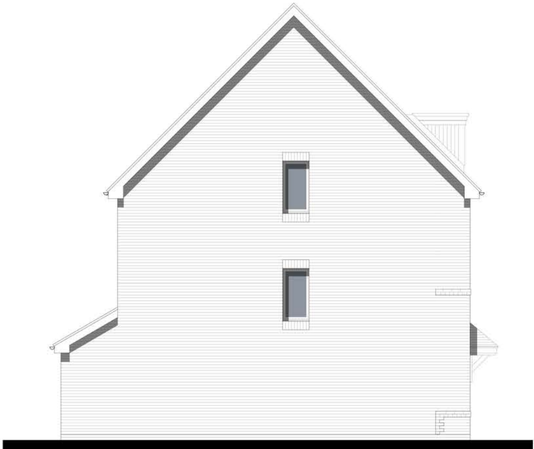
SIDE ELEVATION
