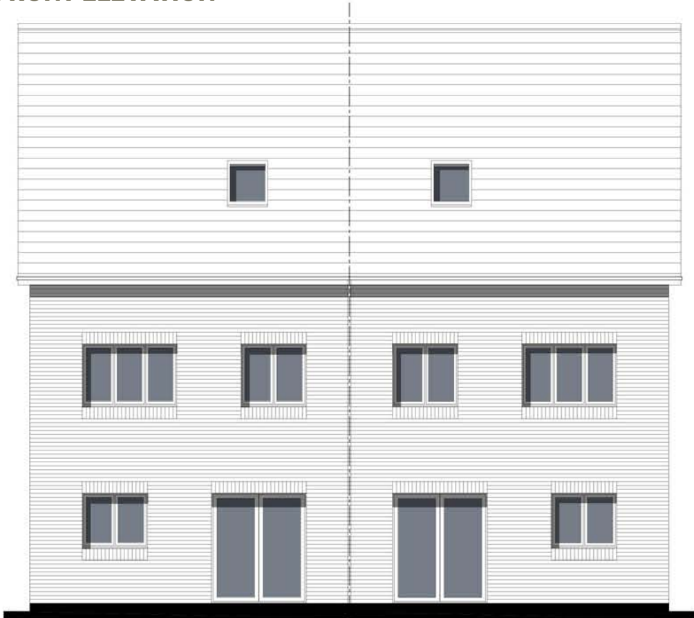
REAR ELEVATION
