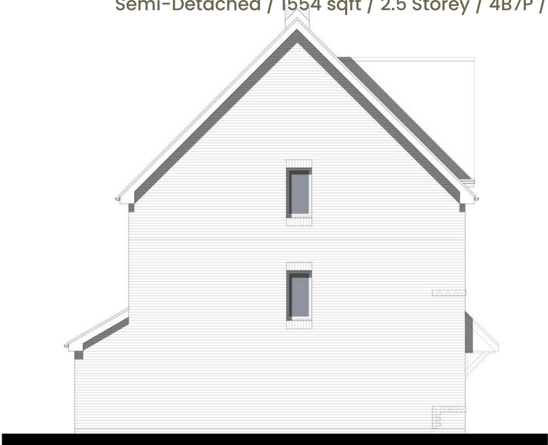
SIDE ELEVATION
