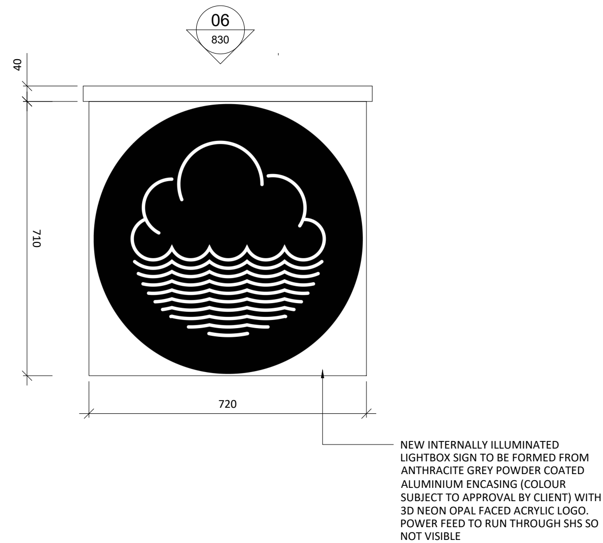
05 ILLUMINATED SIGN AS PROPOSED 830 SCALE - 1:10 @ A1 ELEVATION
