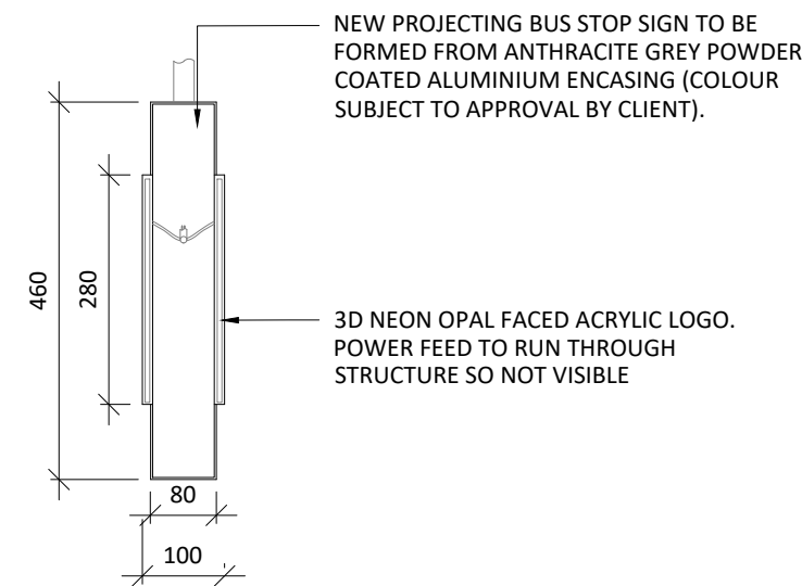
04 ILLUMINATED SIGN AS PROPOSED 830 SCALE - 1:10 @ A1 ELEVATION
