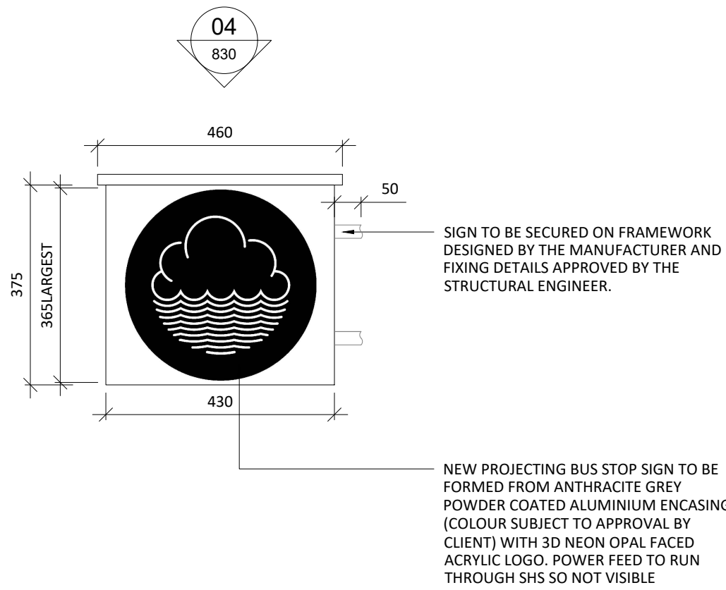
03 ILLUMINATED SIGN AS PROPOSED 830 SCALE - 1:10 @ A1 ELEVATION
