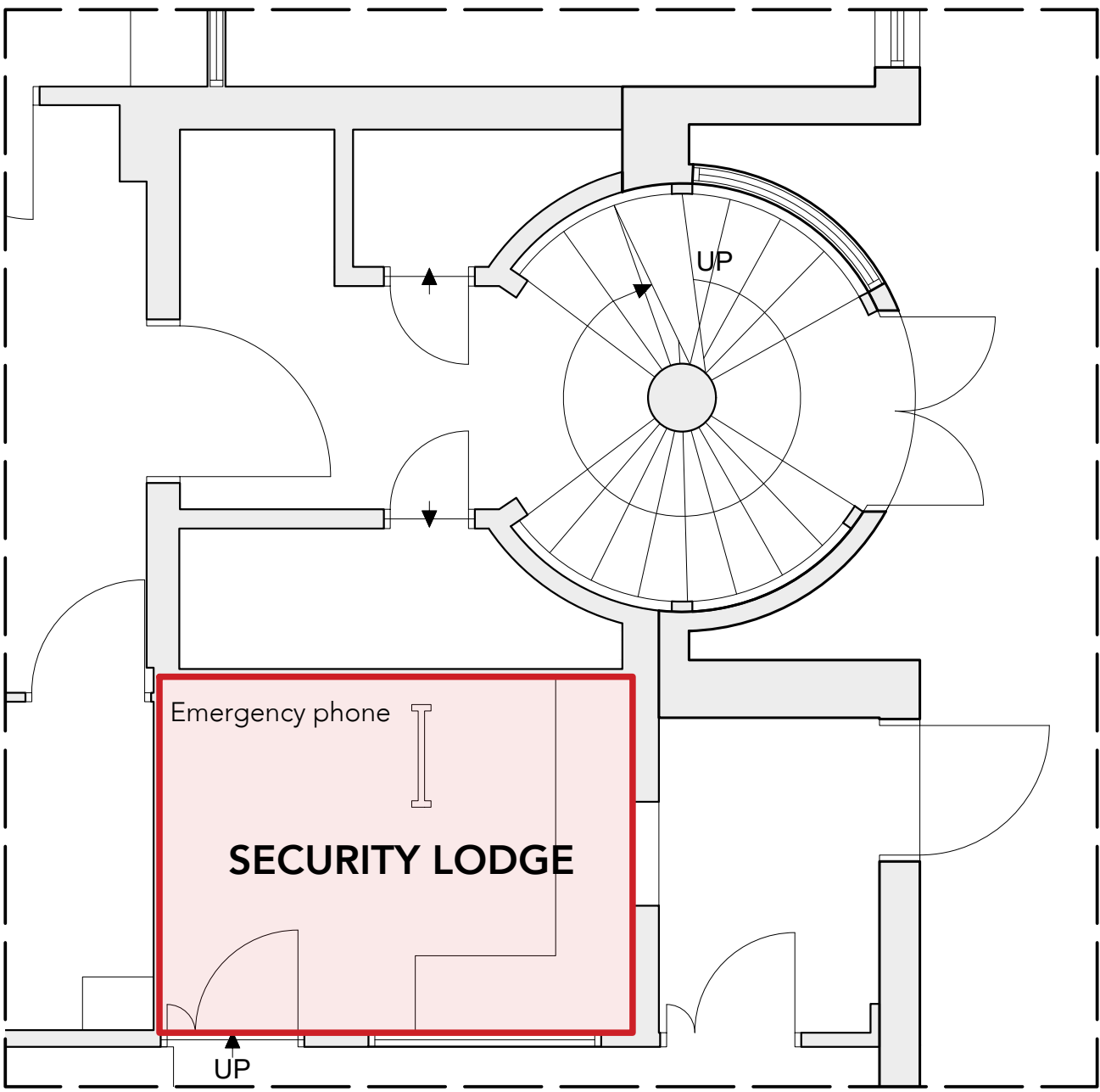
PARTIAL GF PLAN 1:50
