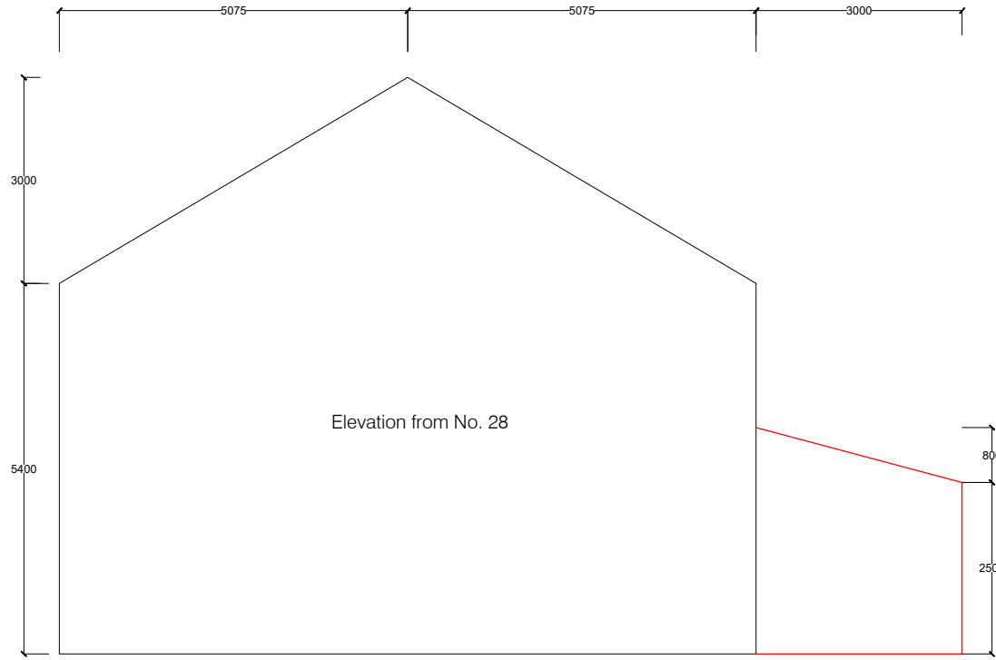
Elevation as Proposed
