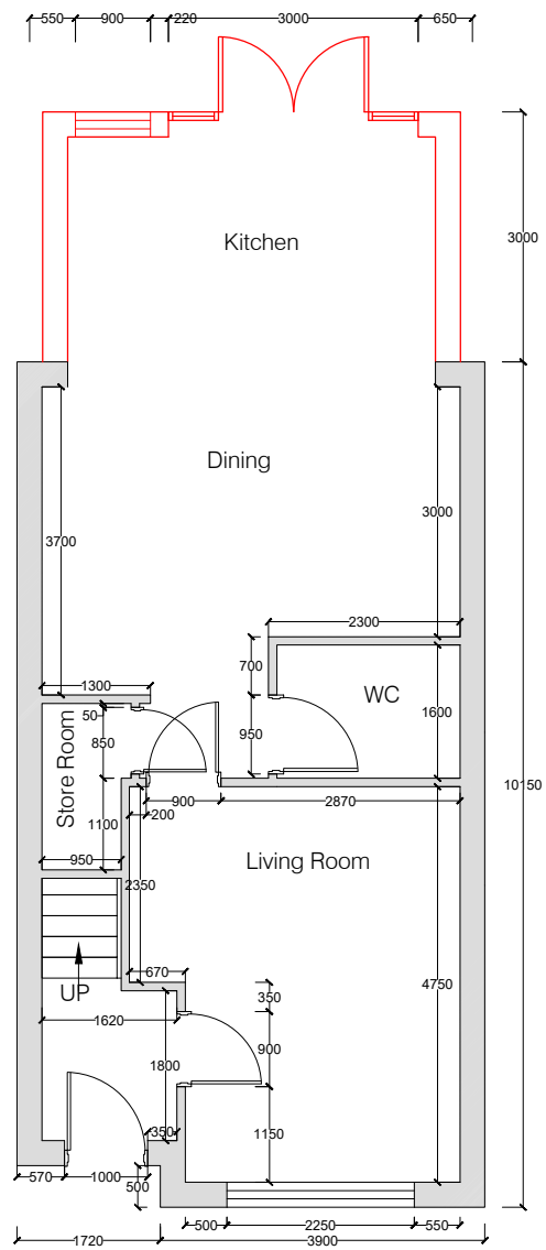
Ground Floor Plan as Proposed
