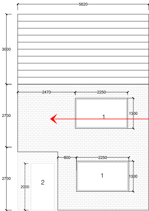
Front Elevation as Proposed
