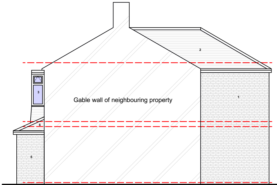
PROPOSED GA SIDE ELEVATION 2
