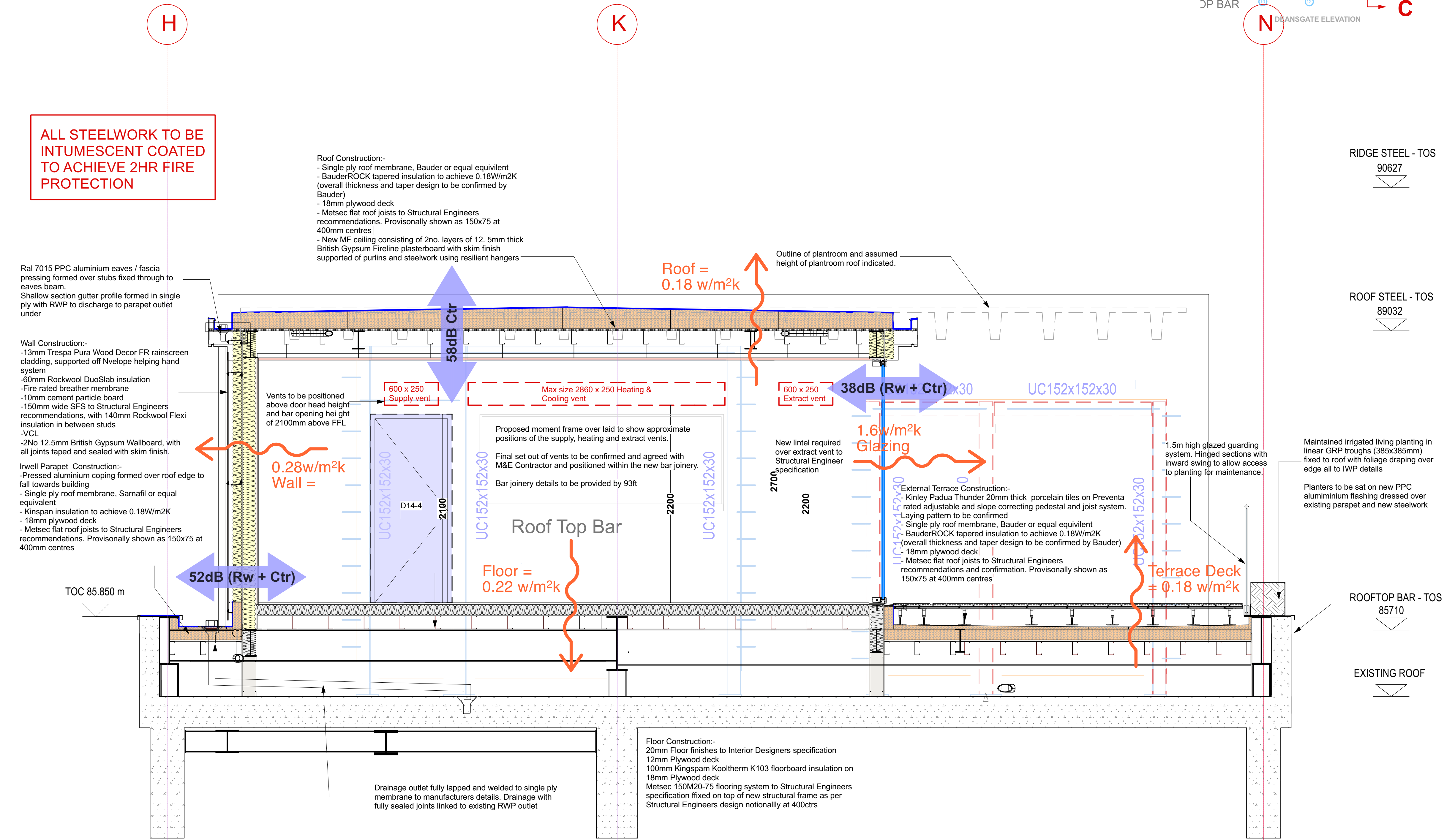
Proposed Roof Terrace Section B-B (1:25@A1)
