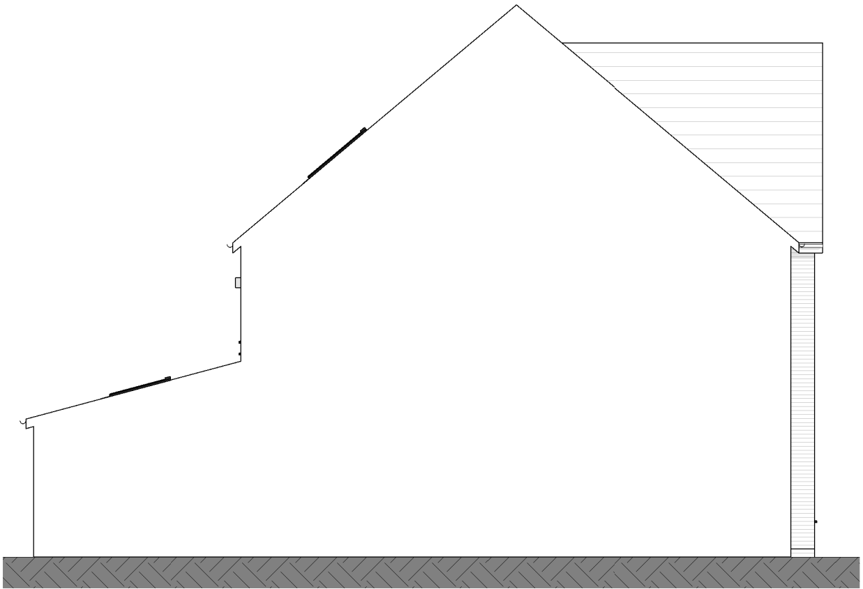
Proposed Side 2 1:100
