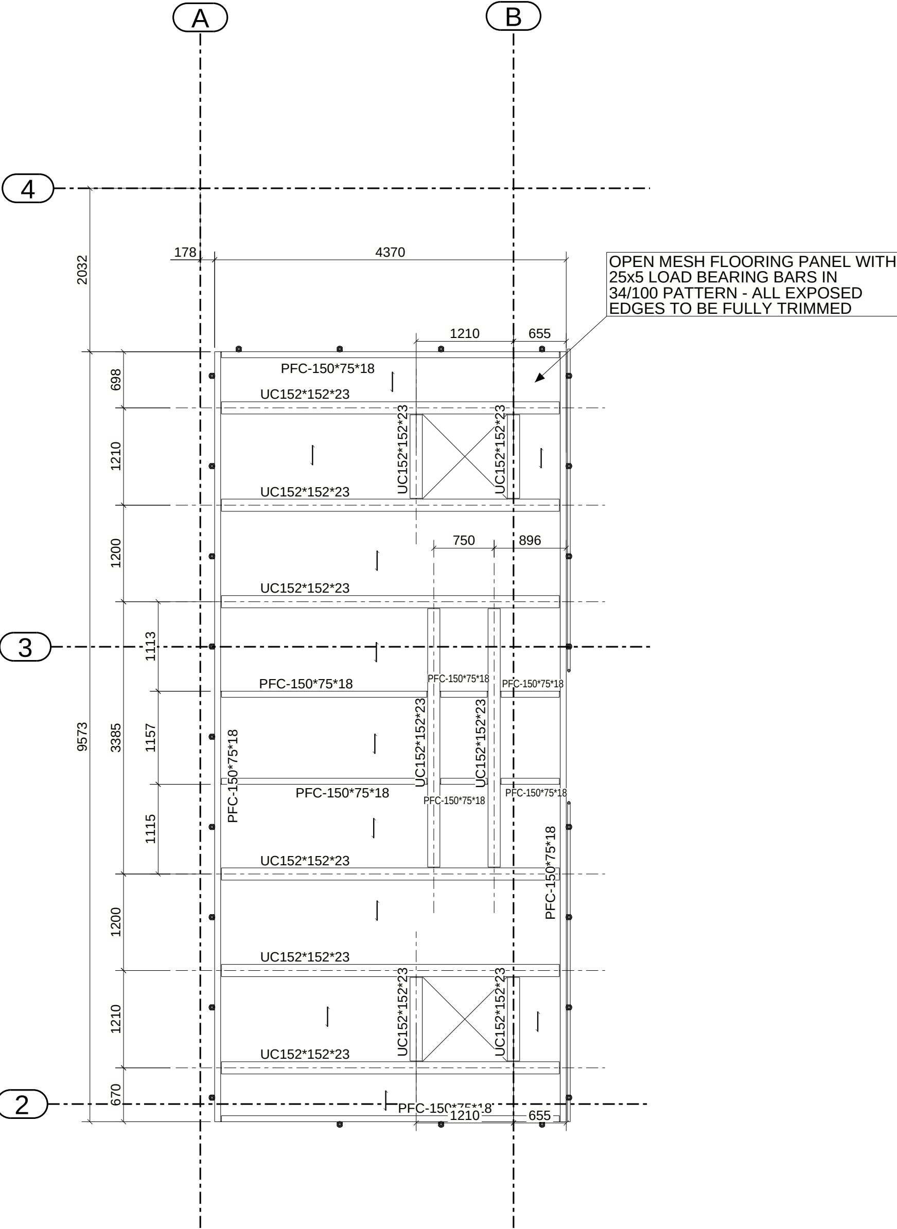
PLAN ON MESH SUPPORT STEEL
