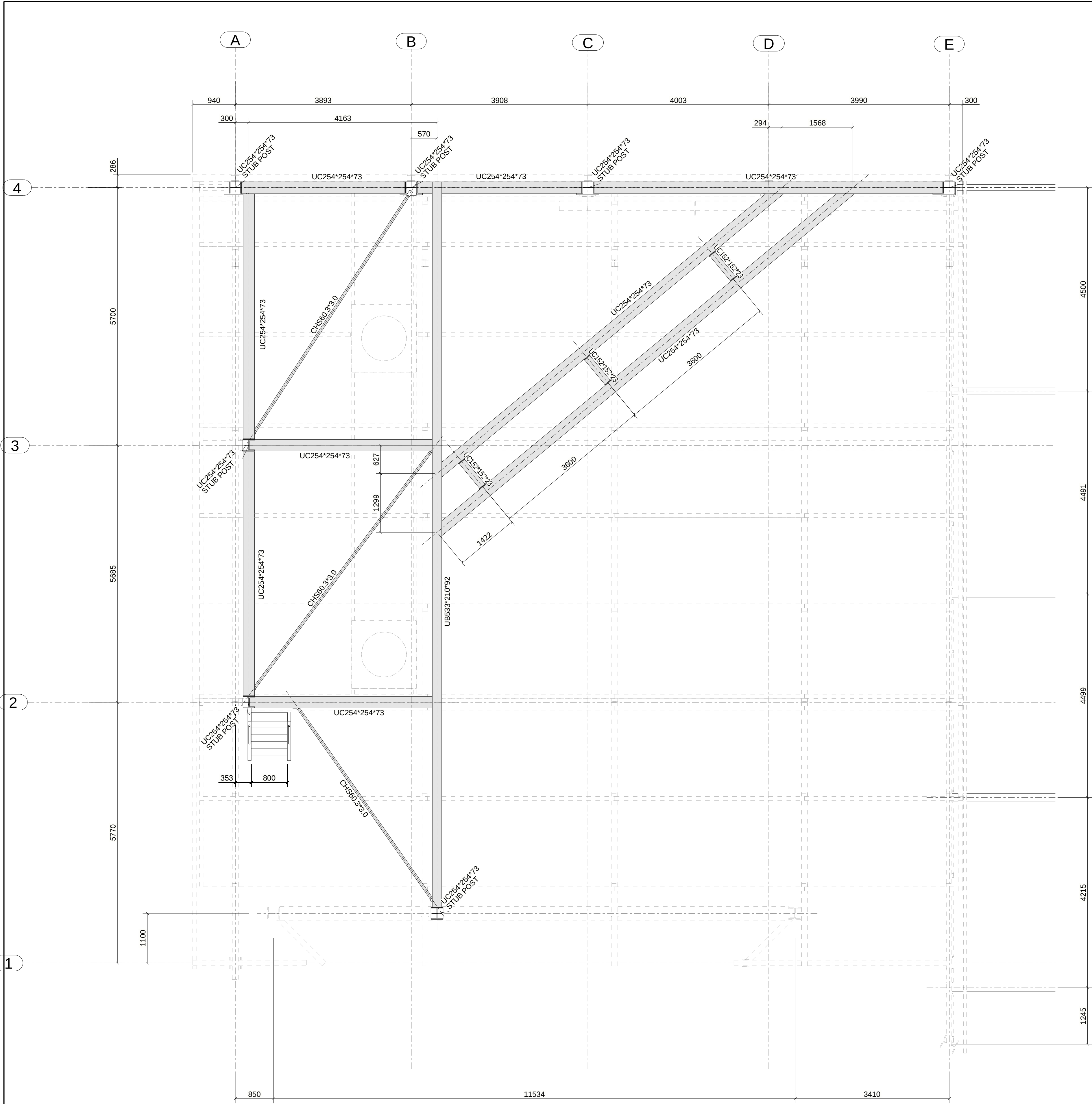
PLAN ON SUB-FRAME
