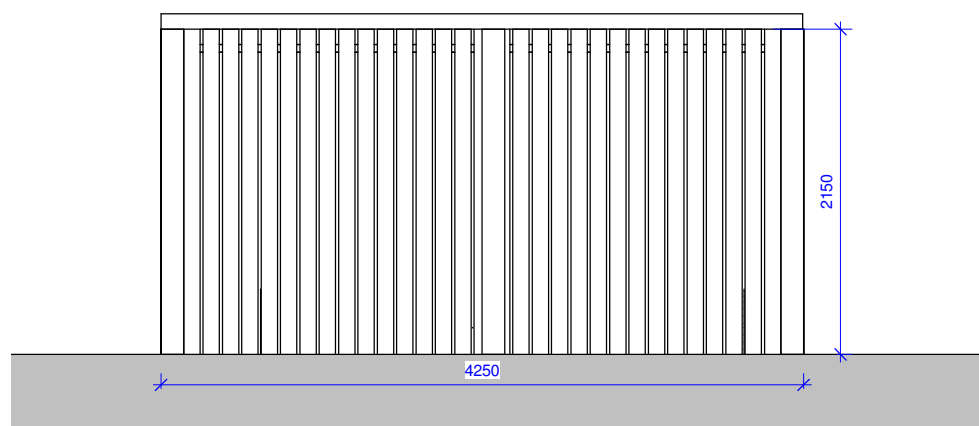
2 Bike Store Elevation 1 : 50
