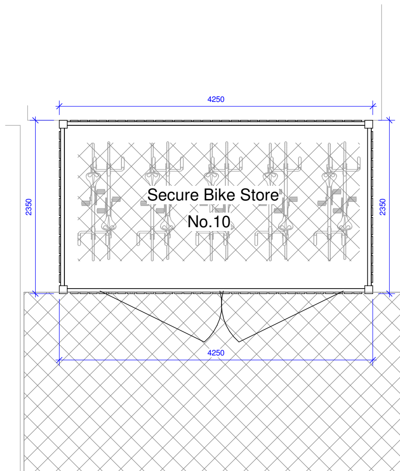
1 Bike Store Plan 1 : 50
