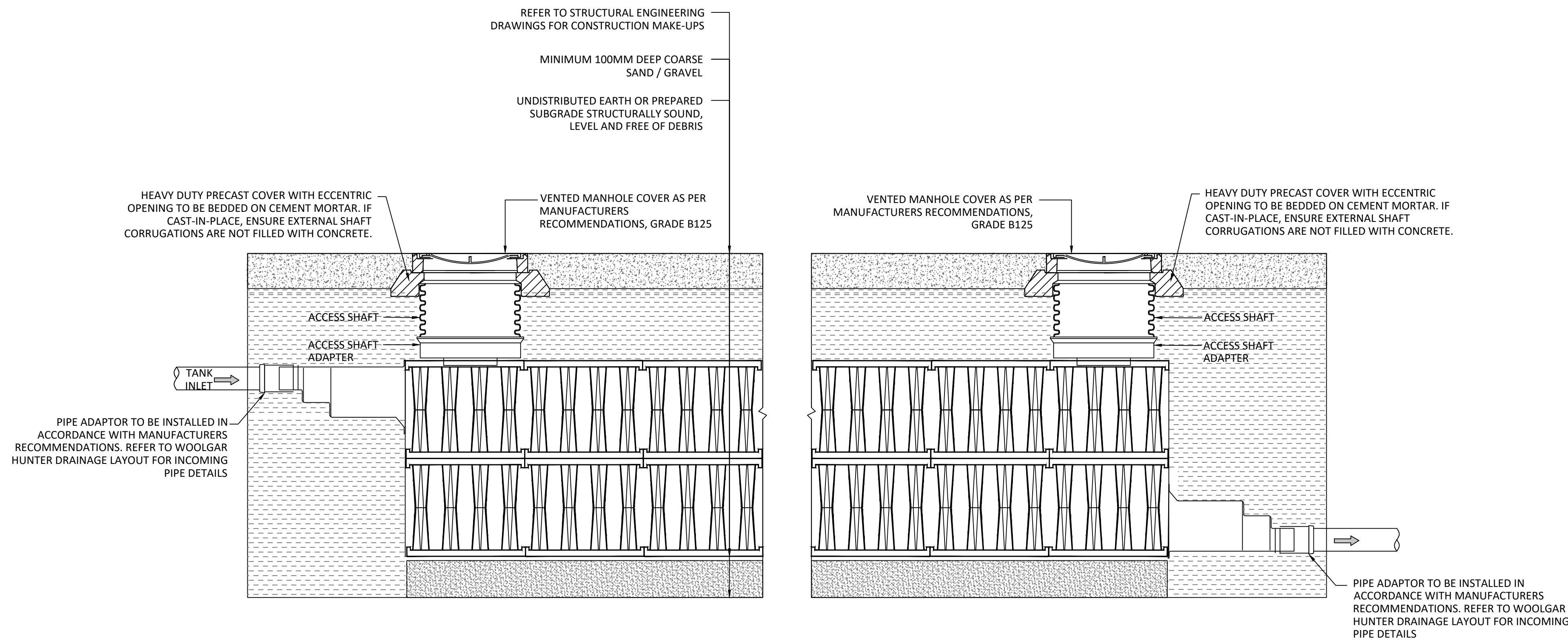
SECTION A TYPICAL STORMBLOC OPTIMUM ATTENUATION TANK
