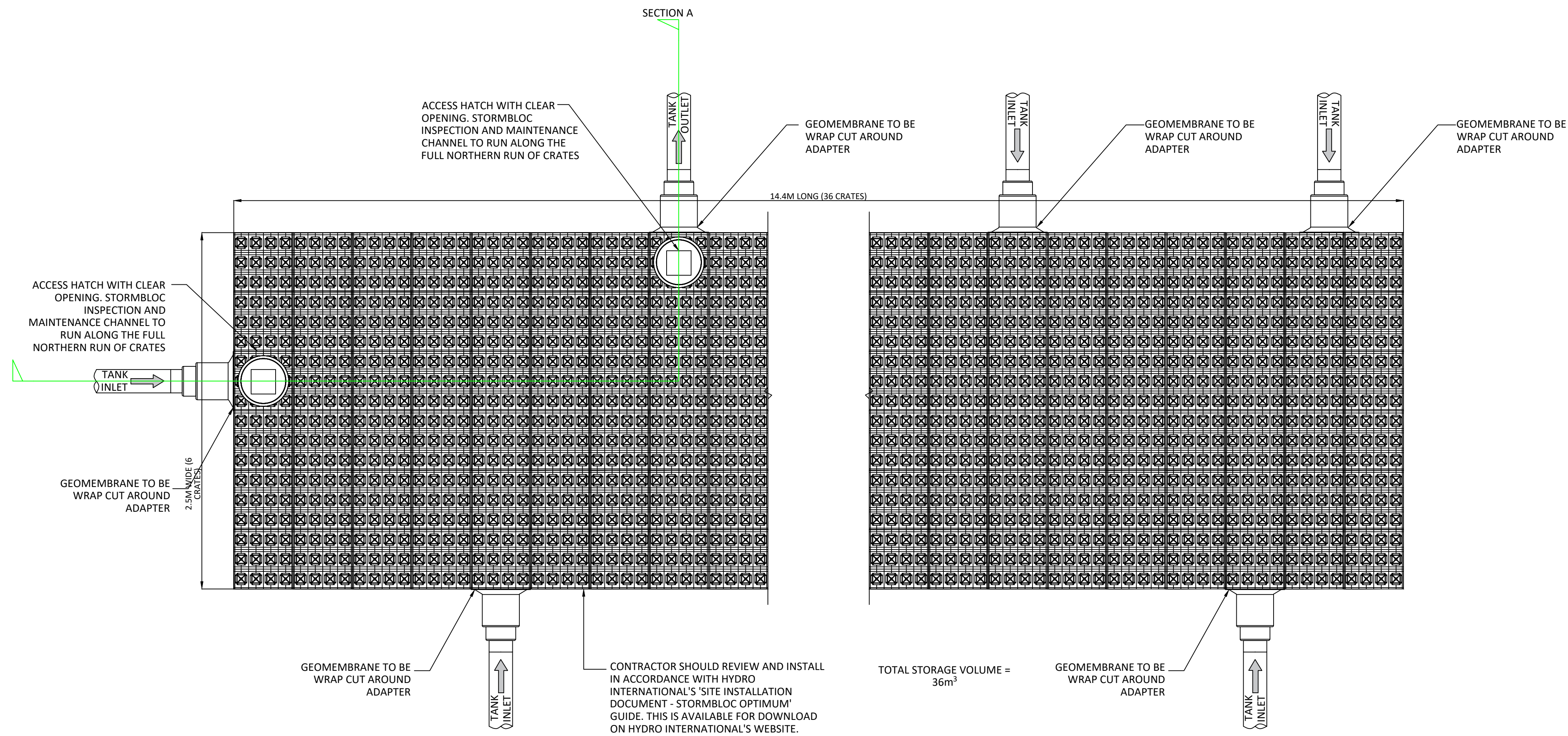
PLAN OF TYPICAL STORMBLOC OPTIMUM ATTENUATION TANK
