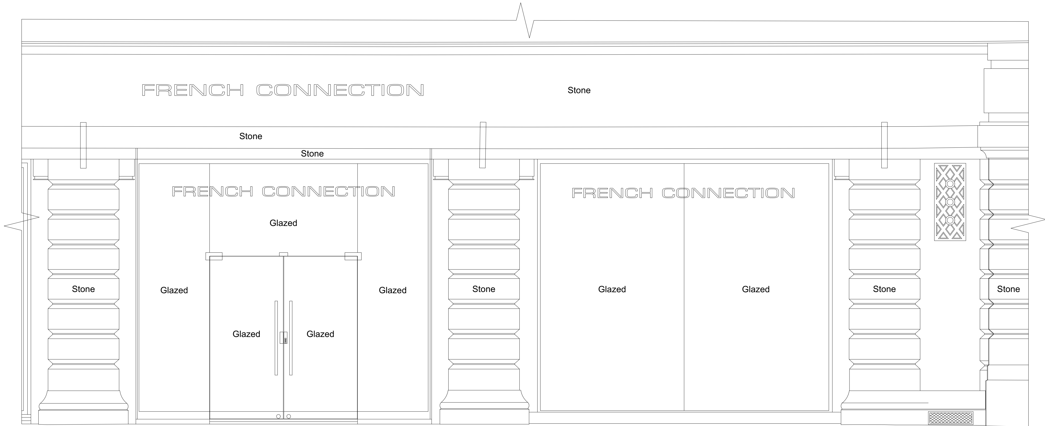
1 EXISTING SHOPFRONT ELEVATION 1:25
