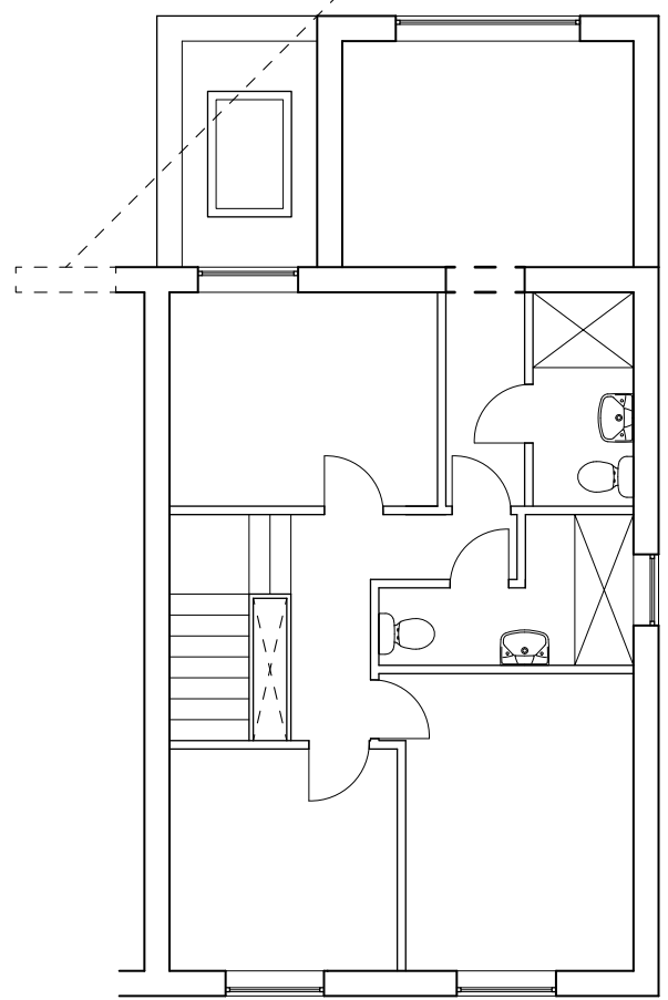
FIRST FLOOR SCALE 1:100 PROPOSED - P004
