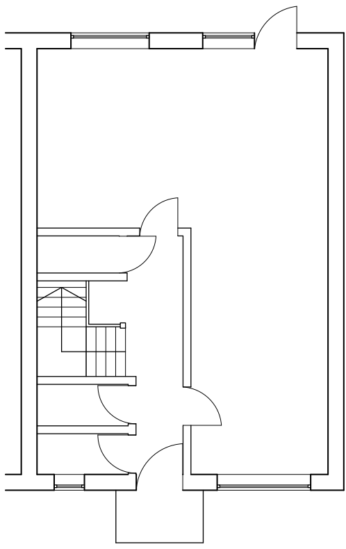
GROUND FLOOR SCALE 1:100 EXISTING - E003
