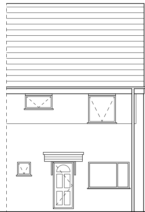
SOUTH EAST ELEVATION SCALE 1:100 PROPOSED - P006
