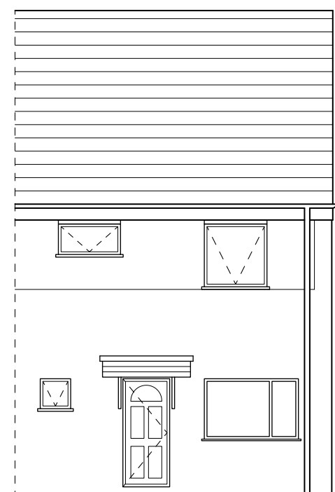
SOUTH EAST ELEVATION SCALE 1:100 EXISTING - E005
