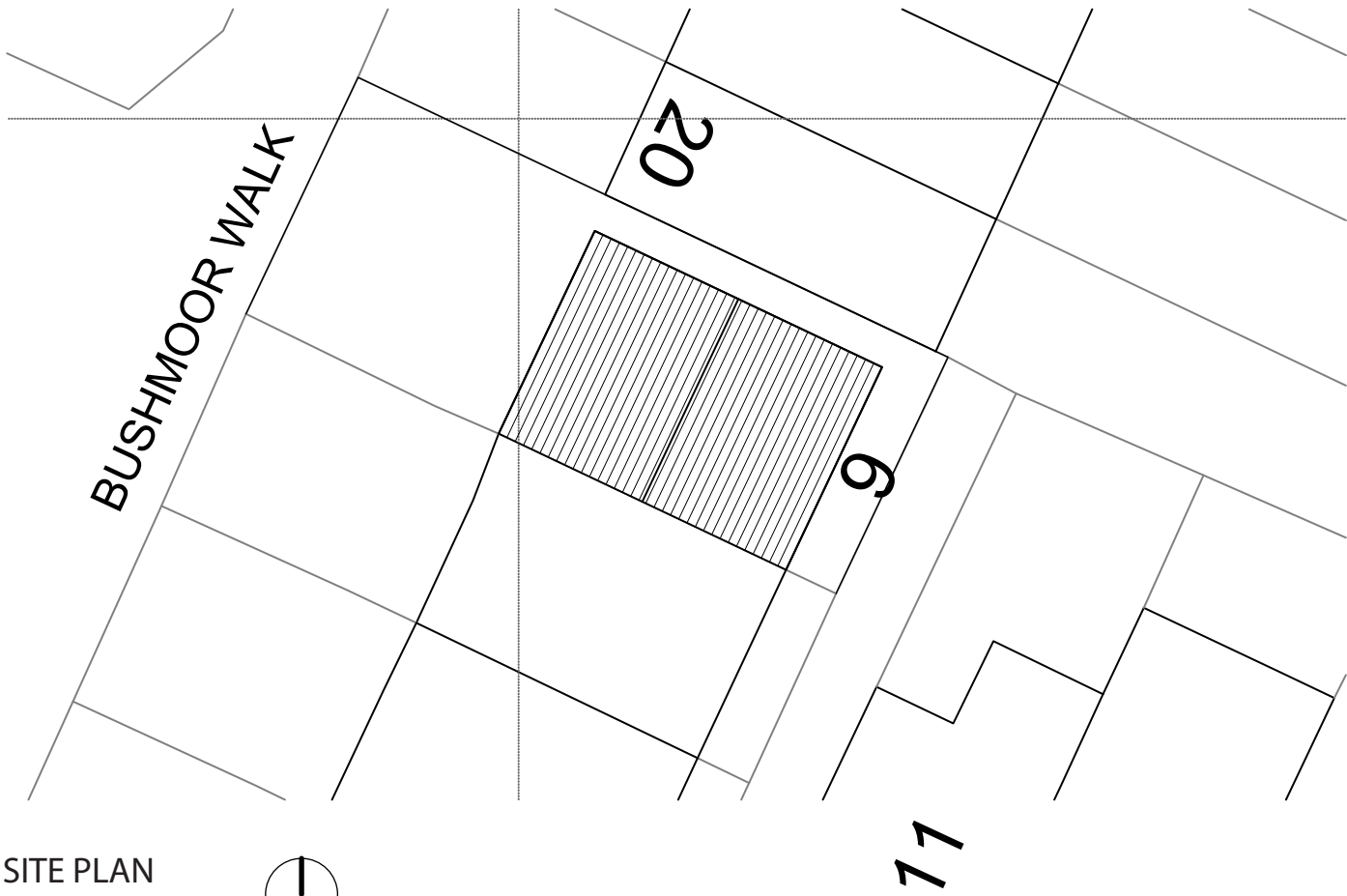
SITE PLAN SCALE 1:200 UID - E001
