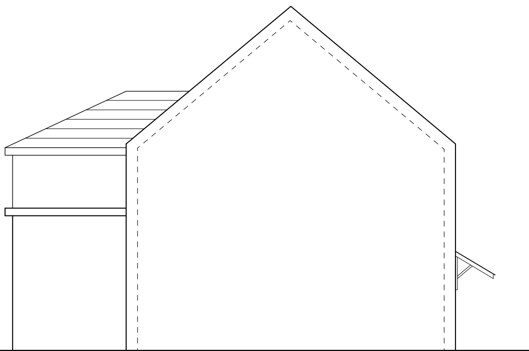
SOUTH WEST ELEVATION SCALE 1:100 PROPOSED - P007
