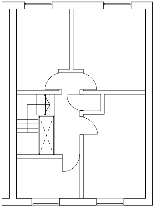
FIRST FLOOR SCALE 1:100 EXISTING - E004
