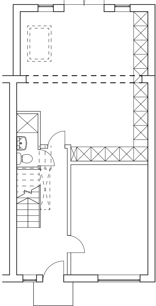
GROUND FLOOR SCALE 1:100 PROPOSED - P003
