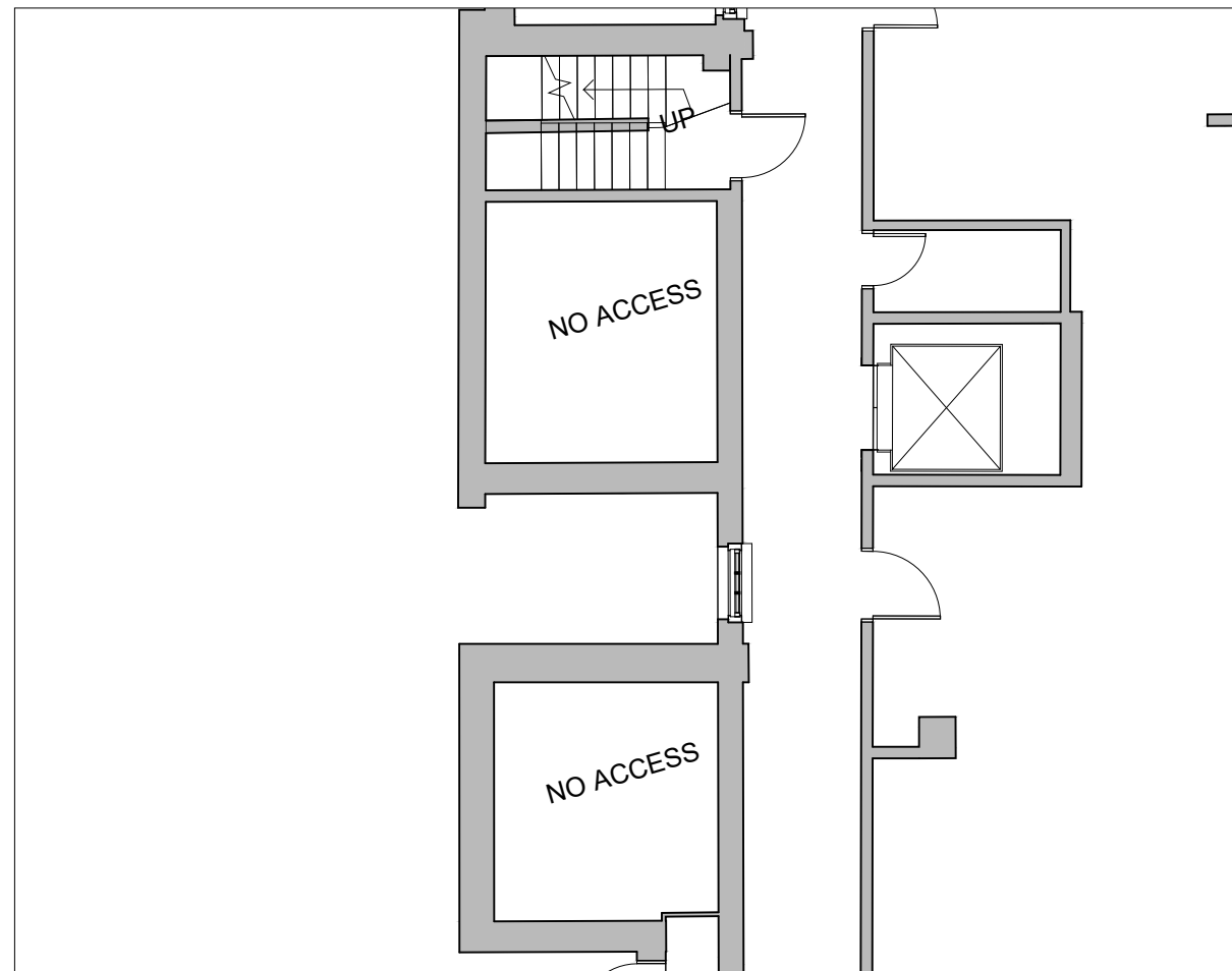
Level 13 WC - 1:100
