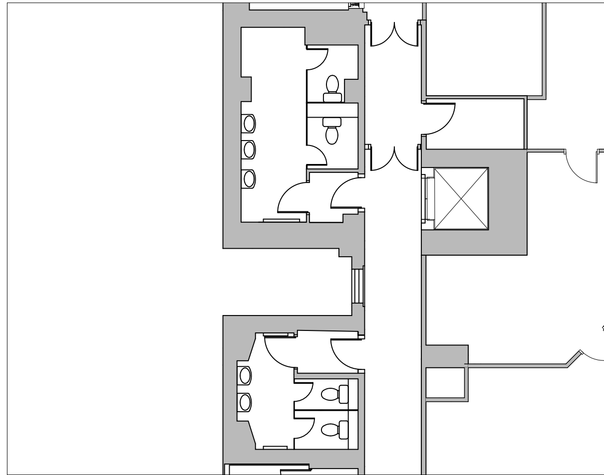
Level 09 WC - 1:100
