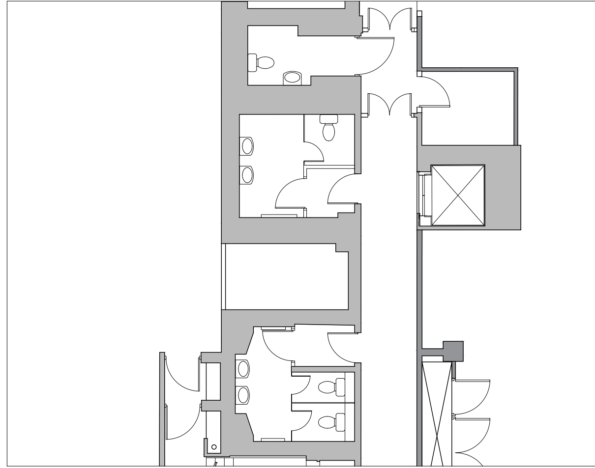
Level 03 WC - 1:100
