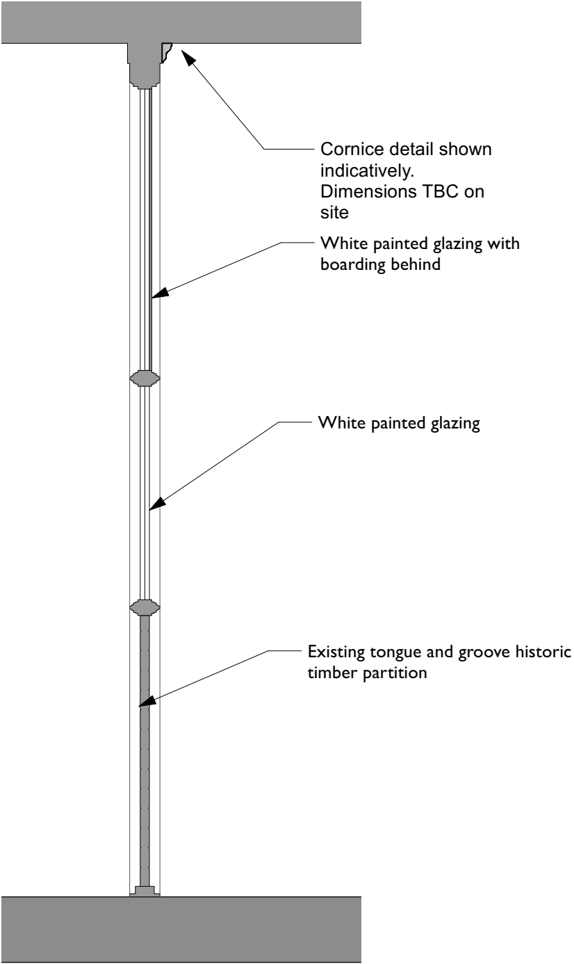
Typical Existing Partition Section AA
