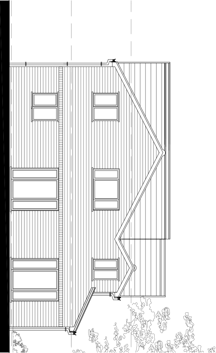
PROPOSED WEST ELEVATION
