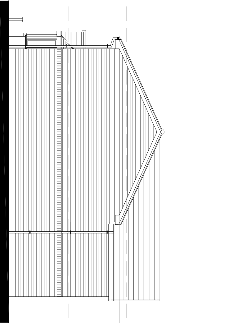
PROPOSED NORTH ELEVATION
