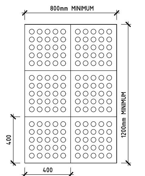
LAYOUT OF TACTILE PAVING
