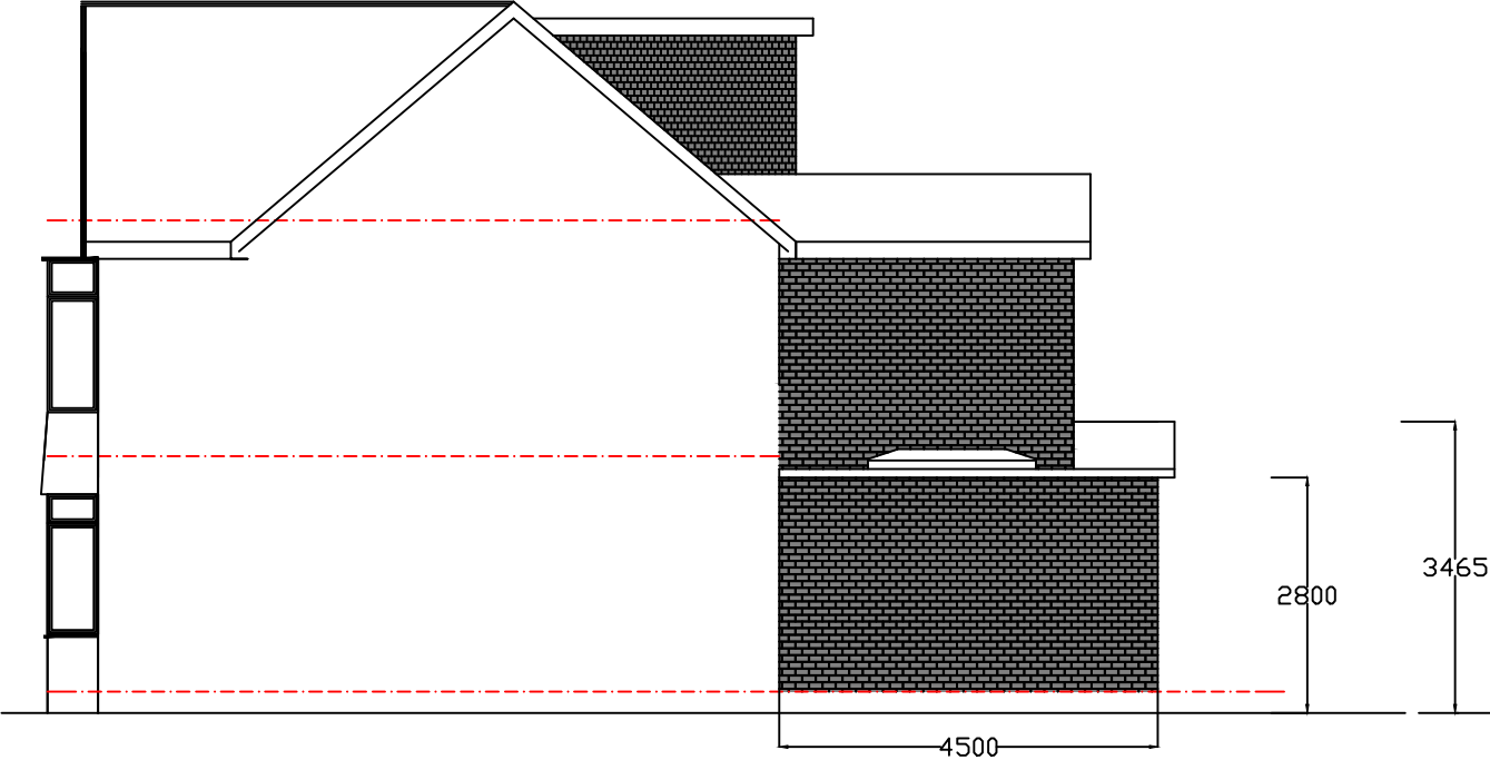
Side Elevation From No 11
