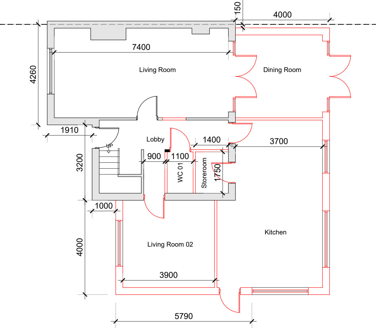
Ground Floor Plan as Proposed
