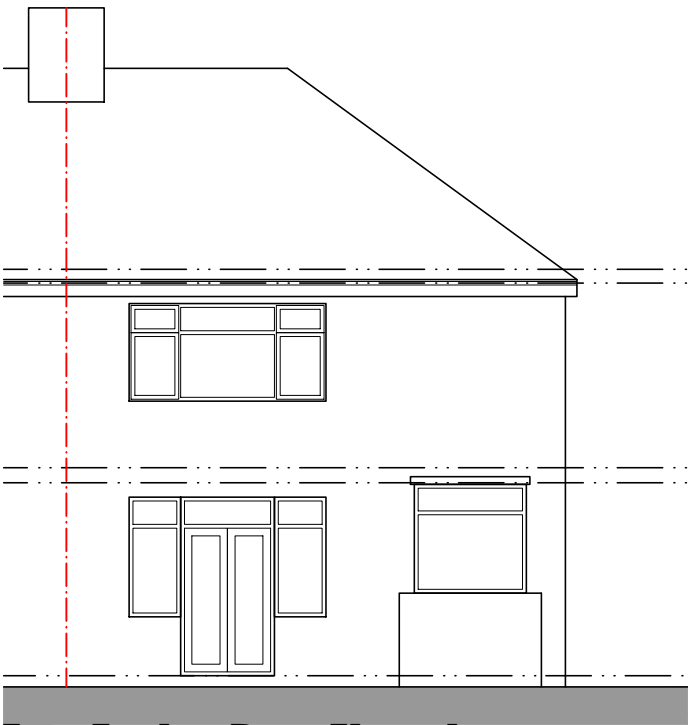
East Facing Rear Elevation
