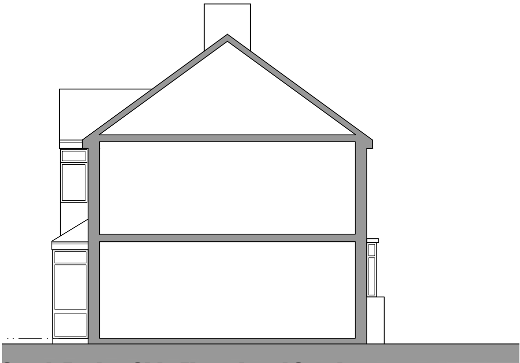
South Facing Side Elevational Section
