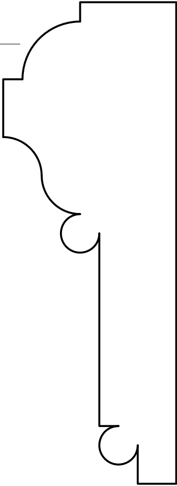
WINDOW SURROUND PROFILE 1:1 @ A3
